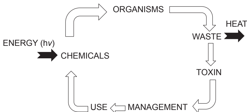
Figure 1. Illustration of the Chemical Feedback during Evolution Adapted from Figure 4.2 from Williams and Rickaby. 2
