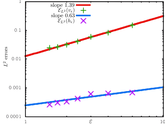
FIGURE 2. The convergence study for L^2 errors of v_\varepsilon and h_\varepsilon in log-log scale. Observed convergence rates are 1.39 for v_\varepsilon , and 0.63 for h_\varepsilon .
