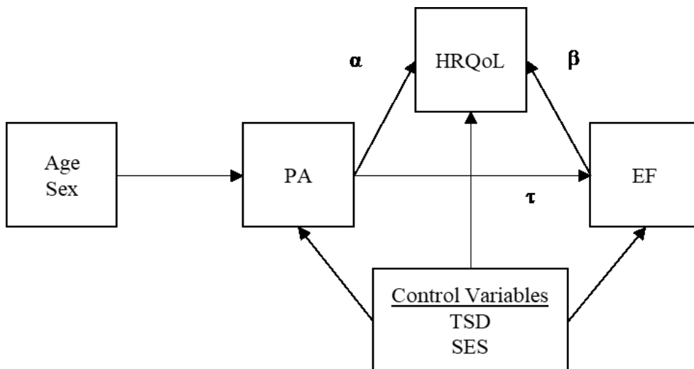
Figure 1. Hypothesized model
