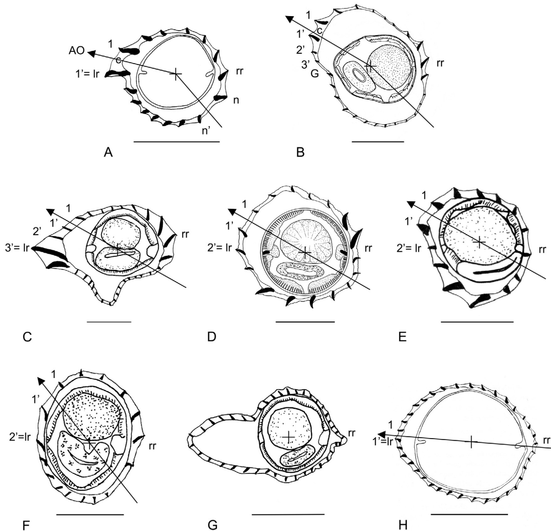
Figure 2. Synlophes at mid-body of the genera treated in this work. Type-species. (A) Odilia ( O. mackerrasae ), male. (B) Hasegawanema n. gen. ( Hasegawanema mamasaense n. comb), female. (C) Hughjonstrongylus ( H. ennisae ), female. (D) Chisholmia n. gen. ( Chisholmia bainae n. comb.), male. (E) Lesleyella n. gen. ( Lesleyella wauensis n. comb.), female. (F) Sanduanensis n. gen. ( Sanduanensis dividua n. comb.), female. (G) Parasabanema ( P. szalayi ), male. (H) Equilophos n. gen. ( Equilophos polyrhabdote n. comb.), female. Abbreviations: 1, 1', 2', 3': ridges 1, 1', 2', 3'; AO: axis of orientation of the ridges; c: careen; G: gap; lr: left ridge; n: last dorsal ridge; n': last ventral ridge; rr: right ridge. A, H, modified from [5]. B, modified from [16]. C, G, modified from [26]. D, modified from [1]. E, modified from [20]. F, modified from [25]. Scale-bars: 50 mm.
