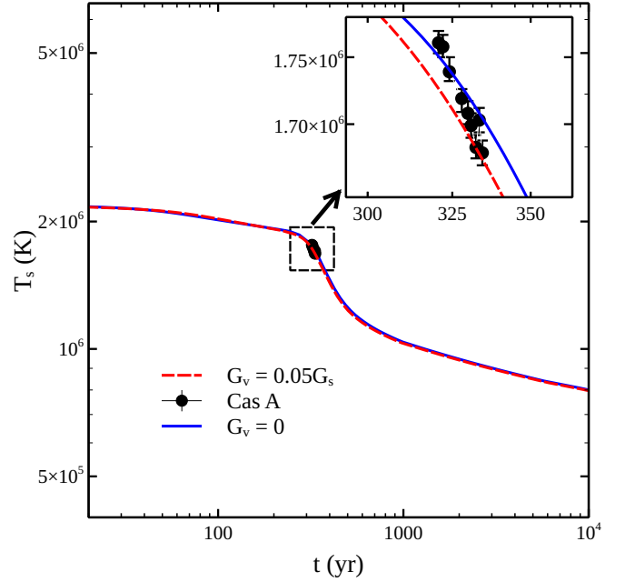
FIG. 6. (Color online) Cooling curves of a M = 1.4 M_{\odot} neutron star computed for NL3 and vector coupling constants G_V = 0 and G_V = 0.05 G_S . The inset shows the data observed for Cas A over a time period of one decade. (Data taken from [70].)
