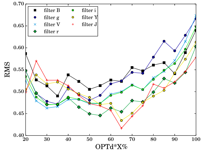
Figure 2. Variation in phase of the dispersion in the Hubble diagram for different filters and using a color term ( V - i ). In the x axis we present the time as (explosion time+OPTd*X%). The black squares represent the B band, dark blue circles the g band, blue crosses the V band, dark green diamonds the r band, green hexagons the i band, yellow pentagons the Y band, and red plus signs the J band. The H band is not represented because the sampling is as good as it is in the other bands.
