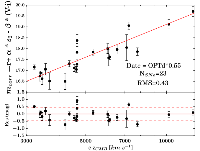
Figure 6. In all the figures, we present the dispersion (rms), the number of SNe ( N_{SNe} ), and the epoch chosen with respect to the end of the plateau (OPTd*X%) for the SCM and with respect to the explosion date for the SCM. On the bottom of each plot, the residuals are shown. In all the residuals plot, the dashed line correspond to the rms. For both methods we use the Hubble flow sample, cz_{CMB} \geq 3000 \text{ km s}^{-1} , the r band and the color ( V - i ). Plotted on the left is the SCM whereas in the right is for the PCM.
