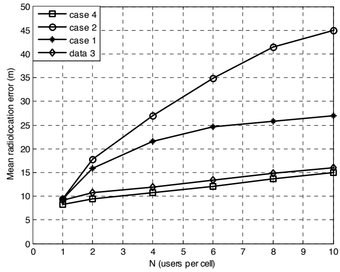
Figure 6.12: Mean radiolocation error vs number of users (DDF)
