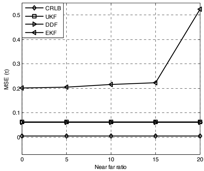
Figure 4.17: The MSE of the time delay estimates versus near-far ratio for three estimators and the CRLB.
