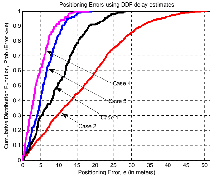
Figure 6.3: Cumulative distribution function (CDF) for the residual mobile positioning error for 4 cases using DDF
