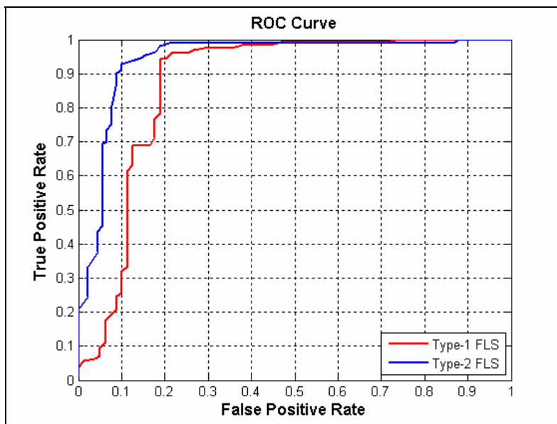
Figure 6-21: ROC Curve during testing of Type-1 and Type-2 FLS on Wisconsin Breast Cancer Dataset
