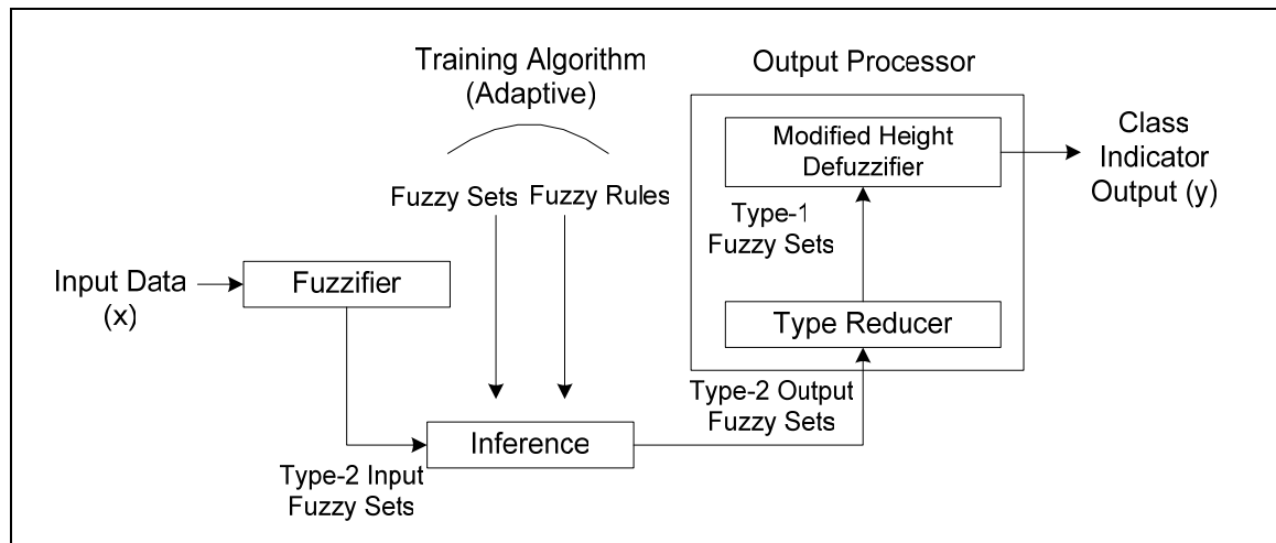
Figure 4-10: Proposed Adaptive FLS Classification Framework
