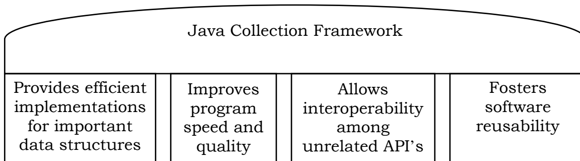
Figure 4: JCF argument
