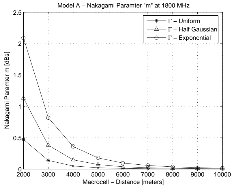
Figure 4.4: Nakagami m variations: Model A, Macrocell, 1800 MHz
