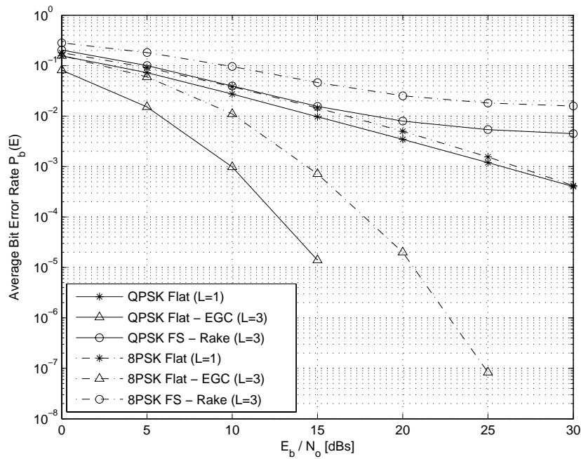
Figure 4.73: MPSK System:Flat fading with EGC and Frequency Selective fading with Rake reception over slowly fading channel, f = 1800MHz , d = 8km , \Gamma Exponential
