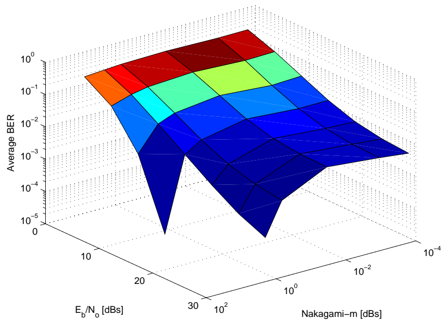
Figure 4.94: Impact of Nakagami- m variations on Average BEP of QPSK with Rake receiver ( L=3 ), f = 900\text{MHz} , \Gamma Exponential
