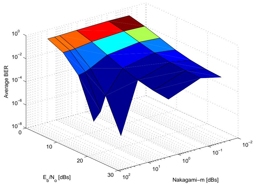
Figure 4.95: Impact of Nakagami- m variations on Average BEP of QPSK with Rake receiver ( L=3 ), f = 1800\text{MHz} , \Gamma Exponential
