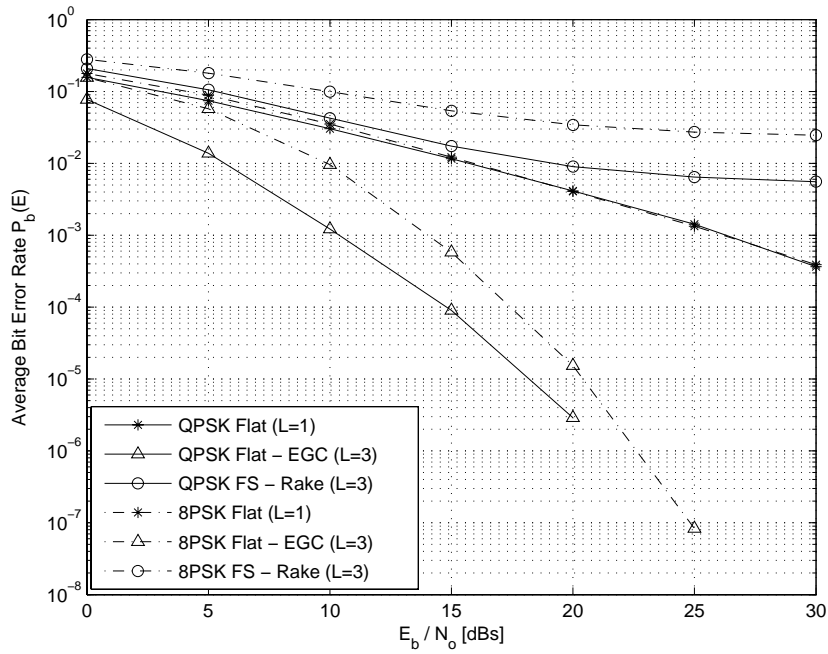
Figure 4.76: MPSK System:Flat fading with EGC and Frequency Selective fading with Rake reception over slowly fading channel, f = 900MHz , d = 5km , \Gamma Half Gaussian
