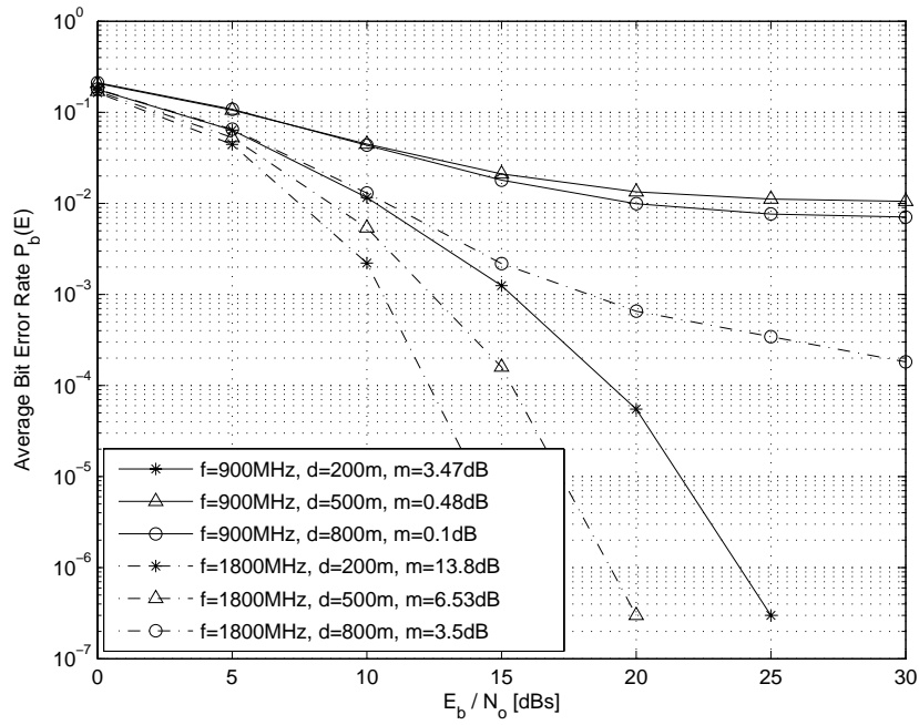
Figure 4.80: Microcell d = 100m - 1km variations of QPSK in microcell over Nakagami- m channel with Rake reception, \Gamma Uniform
