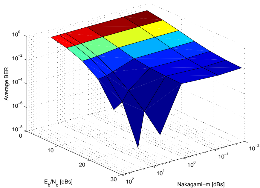
Figure 4.109: Impact of Nakagami- m variations on Average BEP of 8PSK with Rake receiver ( L=3 ), f = 1800\text{MHz} , \Gamma Half Gaussian
