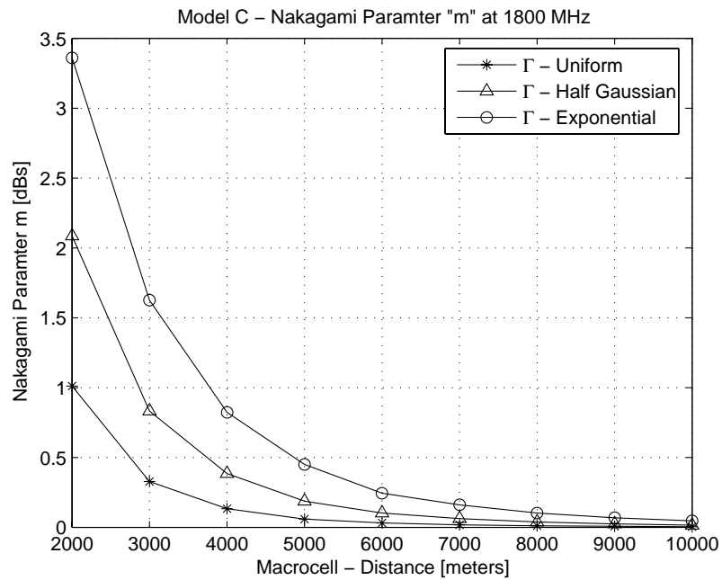
Figure 4.12: Nakagami m variations:Model C, Macrocell, 1800 MHz
