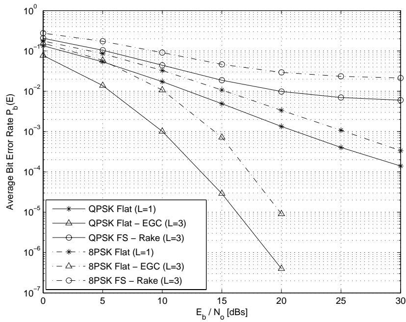
Figure 4.72: MPSK System:Flat fading with EGC and Frequency Selective fading with Rake reception over slowly fading channel, f = 900MHz , d = 8km , \Gamma Exponential
