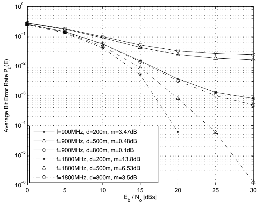
Figure 4.81: Microcell d = 100m - 1km variations of 8PSK in microcell over Nakagami- m channel with Rake reception, \Gamma Uniform
