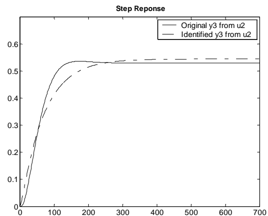
Figure 3.122 : Case 2- Step response of Output-3 from Input-2 (State space)
