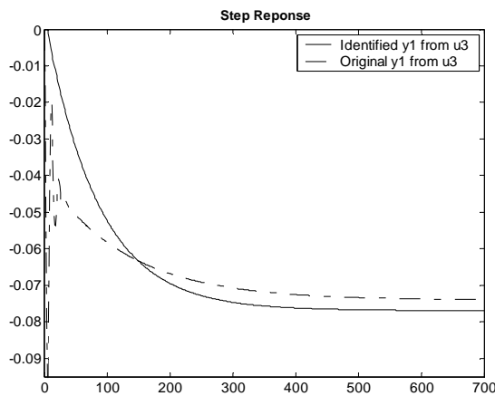
Figure 3.179 : Case 3- Step response of Output-1 from Input-3 (State space)
