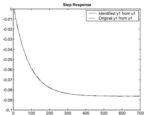
Figure 3.145 : Case 3- Step response of Output-1 from Input-1 (ARMAX)
