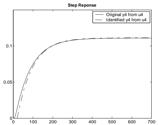
Figure 3.32 : Case 1- Step response of Output-4 from Input-4 (ARMAX)
