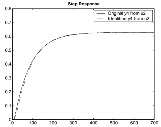
Figure 4.38 : Step Responses of the Actual Open Loop and Identified ARMAX models (Output-4 from Input-2)
