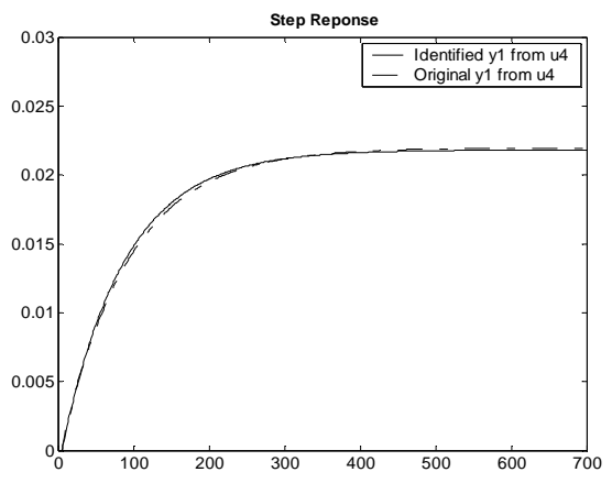
Figure 3.132 : Case 3- Step response of Output-1 from Input-4 (ARX)
