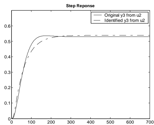
Figure 3.26 : Case 1- Step response of Output-3 from Input-2 (ARMAX)
