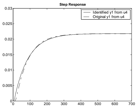
Figure 4.28 : Step Responses of the Actual Open Loop and Identified ARMAX models (Output-1 from Input-4)
