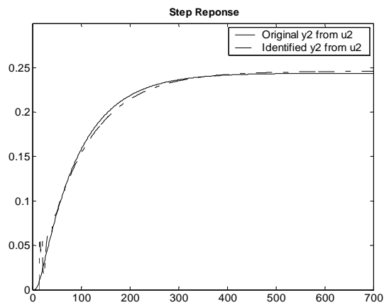
Figure 3.134 : Case 3- Step response of Output-2 from Input-1 (ARX)
