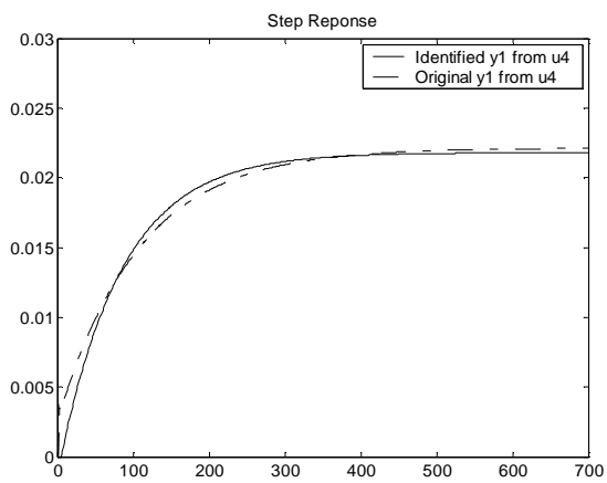
Figure 3.4 : Case 1- Step response of Output-1 from Input-4 (ARX)
