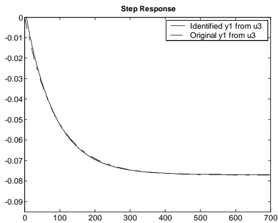
Figure 3.83 : Case 2- Step response of Output-1 from Input-3 (ARMAX)
