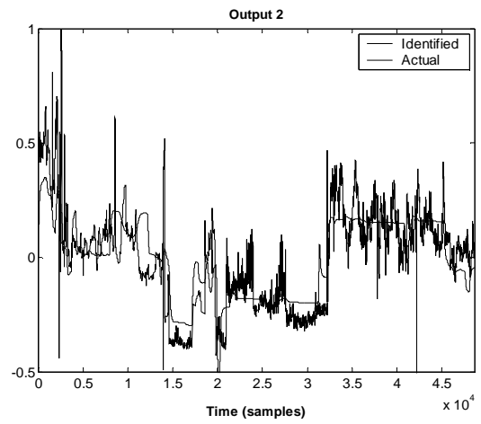
Figure 4.22: Responses of Output 2 Actual and Identified ARMAX Model
