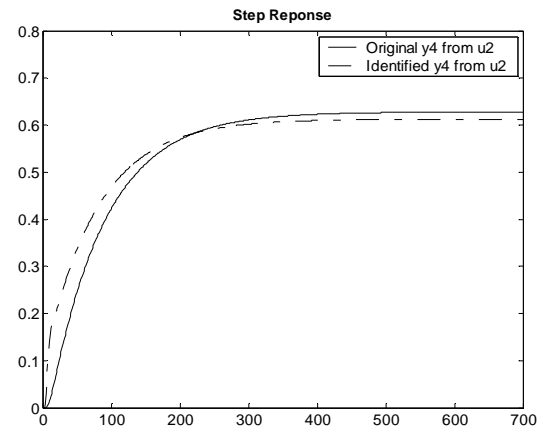
Figure 3.30 : Case 1- Step response of Output-4 from Input-2 (ARMAX)
