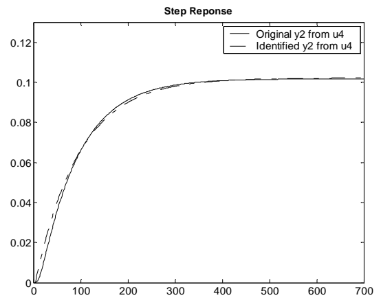
Figure 3.8 : Case 1- Step response of Output-2 from Input-4 (ARX)
