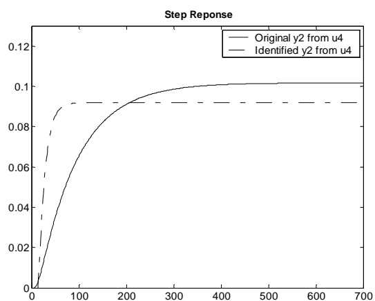
Figure 3.104 : Case 2- Step response of Output-2 from Input-4 (OE)
