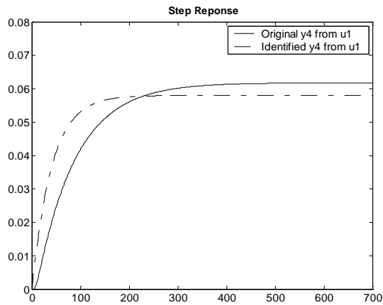
Figure 3.61 : Case 1- Step response of Output-4 from Input-1 (State space)
