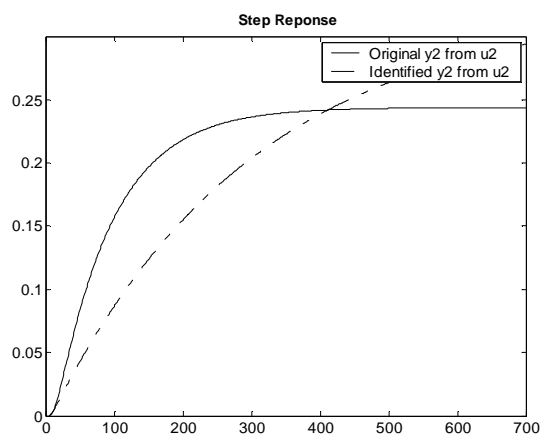
Figure 3.102 : Case 2- Step response of Output-2 from Input-2 (OE)
