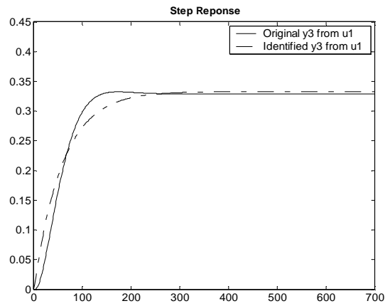
Figure 4.13 : Step Responses of the Actual Open Loop and Identified ARX models (Output-3 from Input-1)
