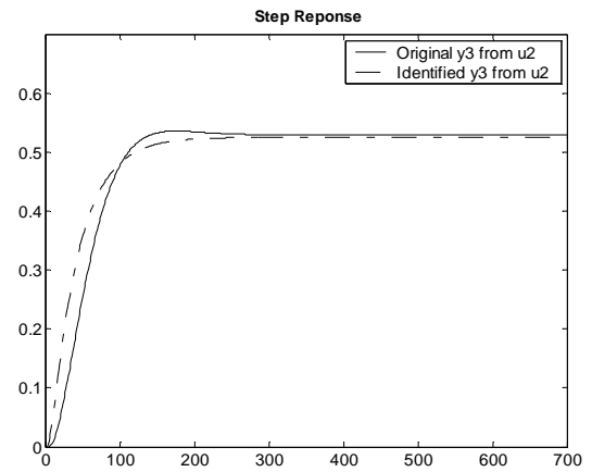
Figure 3.106 : Case 2- Step response of Output-3 from Input-2 (OE)
