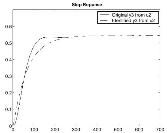
Figure 3.74 : Case 2- Step response of Output-3 from Input-2 (ARX)
