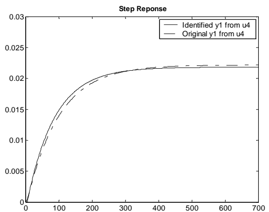
Figure 4.8 : Step Responses of the Actual Open Loop and Identified ARX models (Output-1 from Input-4)
