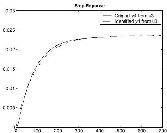
Figure 3.143 : Case 3- Step response of Output-4 from Input-3 (ARX)
