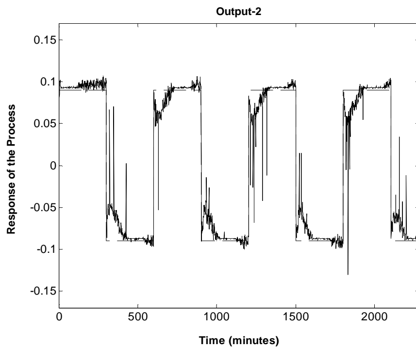
Figure 2.39: Case 1 - Response of MPC (Output-2)
