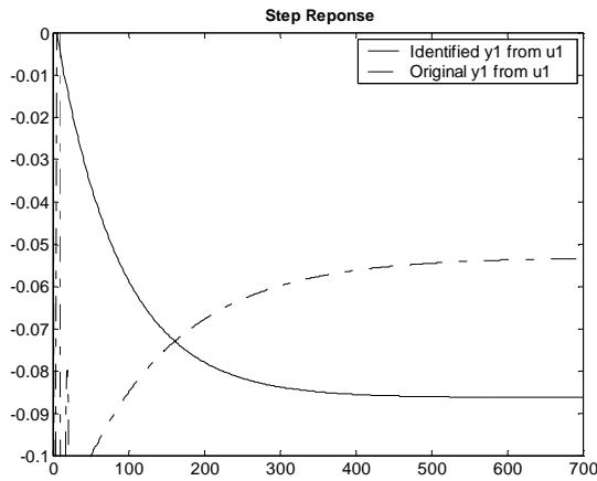
Figure 3.177 : Case 3- Step response of Output-1 from Input-1 (State space)
