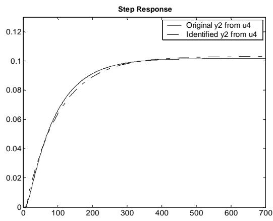
Figure 3.152 : Case 3- Step response of Output-2 from Input-4 (ARMAX)
