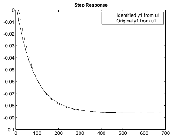
Figure 4.25: Step Responses of the Actual Open Loop and Identified ARMAX models (Output-1 from Input-1)
