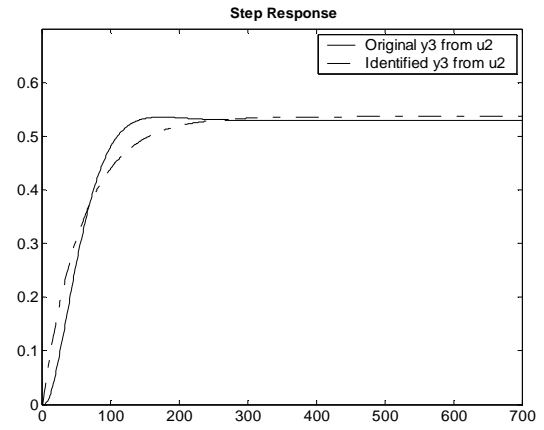
Figure 3.154 : Case 3- Step response of Output-3 from Input-2 (ARMAX)
