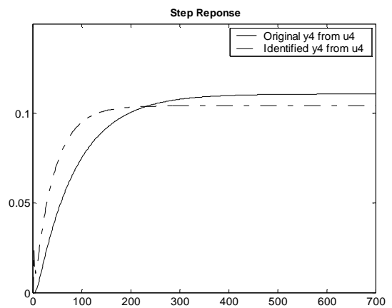
Figure 3.64 : Case 1- Step response of Output-4 from Input-4 (State space)
