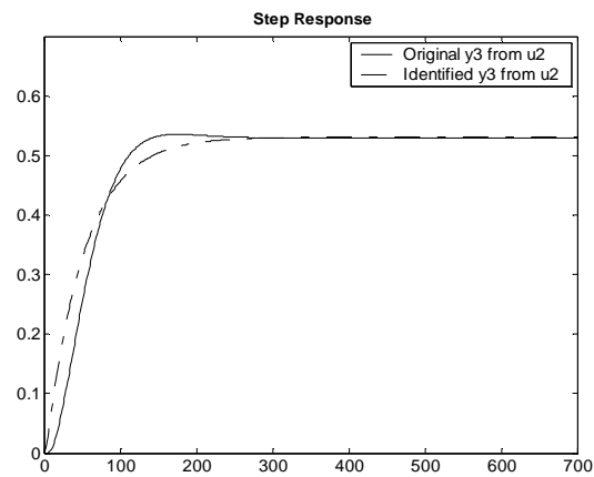
Figure 4.34 : Step Responses of the Actual Open Loop and Identified ARMAX models (Output-3 from Input-2)
