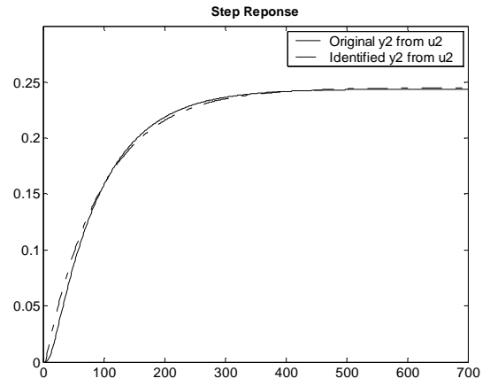
Figure 3.6 : Case 1- Step response of Output-2 from Input-2 (ARX)
