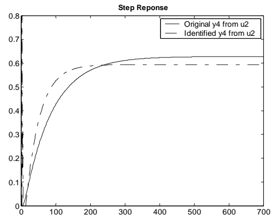
Figure 3.62 : Case 1- Step response of Output-4 from Input-2 (State space)
