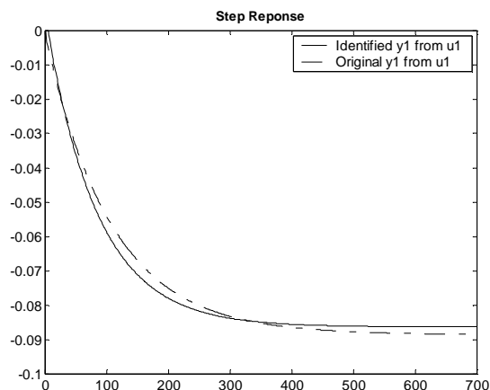
Figure 3.1 : Case 1- Step response of Output-1 from Input-1 (ARX)
