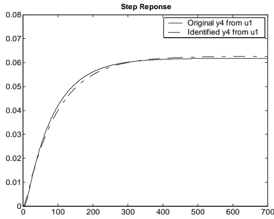
Figure 4.17 : Step Responses of the Actual Open Loop and Identified ARX models (Output-4 from Input-1)
