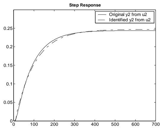
Figure 3.150 : Case 3- Step response of Output-2 from Input-2 (ARMAX)
