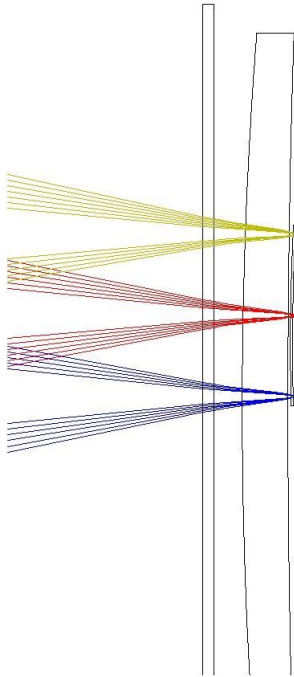
Figure 2. ZTF cryostat raytrace showing the spectral filter just outside the dewar, followed by the hierarchical field-flattening solution: the spherical window, individual field-flattening lenses assigned to each CCD, and a spherically tangent CCD mounting plate.
