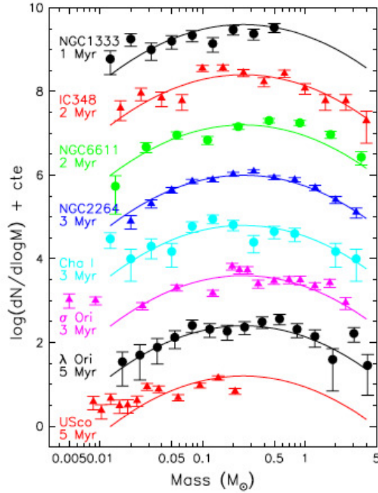
Figure 1: Recent IMF estimates for 8 star forming regions. The error bars represent the Poisson error for each data point. The solid lines are the log-normal form proposed by Chabrier (2005) for the IMF, normalized to best follow the data. From Offner et al. (2014).
