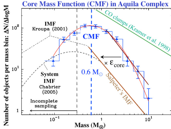
Figure 2: Core mass function (histogram with error bars) of the prestellar cores identified with Herschel in Aquila (Konyves et al. 2015; André et al. 2010). The Kroupa and Chabrier IMF and the typical mass spectrum of CO clumps is shown for comparison.
