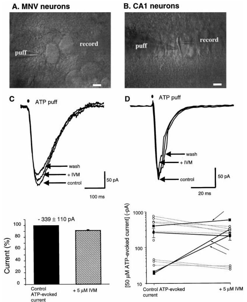
Figure 7. Endogenous P2X channels in MNV and hippocampal CA1 neurons. A , Bright-field image of a brainstem slice containing the MNV. MNV neurons can be seen as round neurons. Scale bar, 10 \mu\text{m} . B , Image of the CA1 region in a hippocampal slice. CA1 pyramidal neurons can be seen extending a dendrite into the stratum radiatum. Scale bar, 10 \mu\text{m} . C , Representative ATP-evoked currents from an MNV neuron. D , Representative traces of ATP-evoked currents from a CA1 neuron. In both cases recordings in the presence of 2–5 \mu\text{M} IVM are also shown. The bar graph represents average values for MNV neurons ( n = 3 ), whereas the scatter graph shows data for nonresponding CA1 neurons ( \circ ), the three responding neurons ( \blacksquare ; arrows), and the average for all 13 neurons ( \bullet ).
