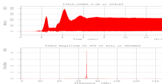
Figure 2: Predicted output power, top, and frequency of output signal, bottom.
