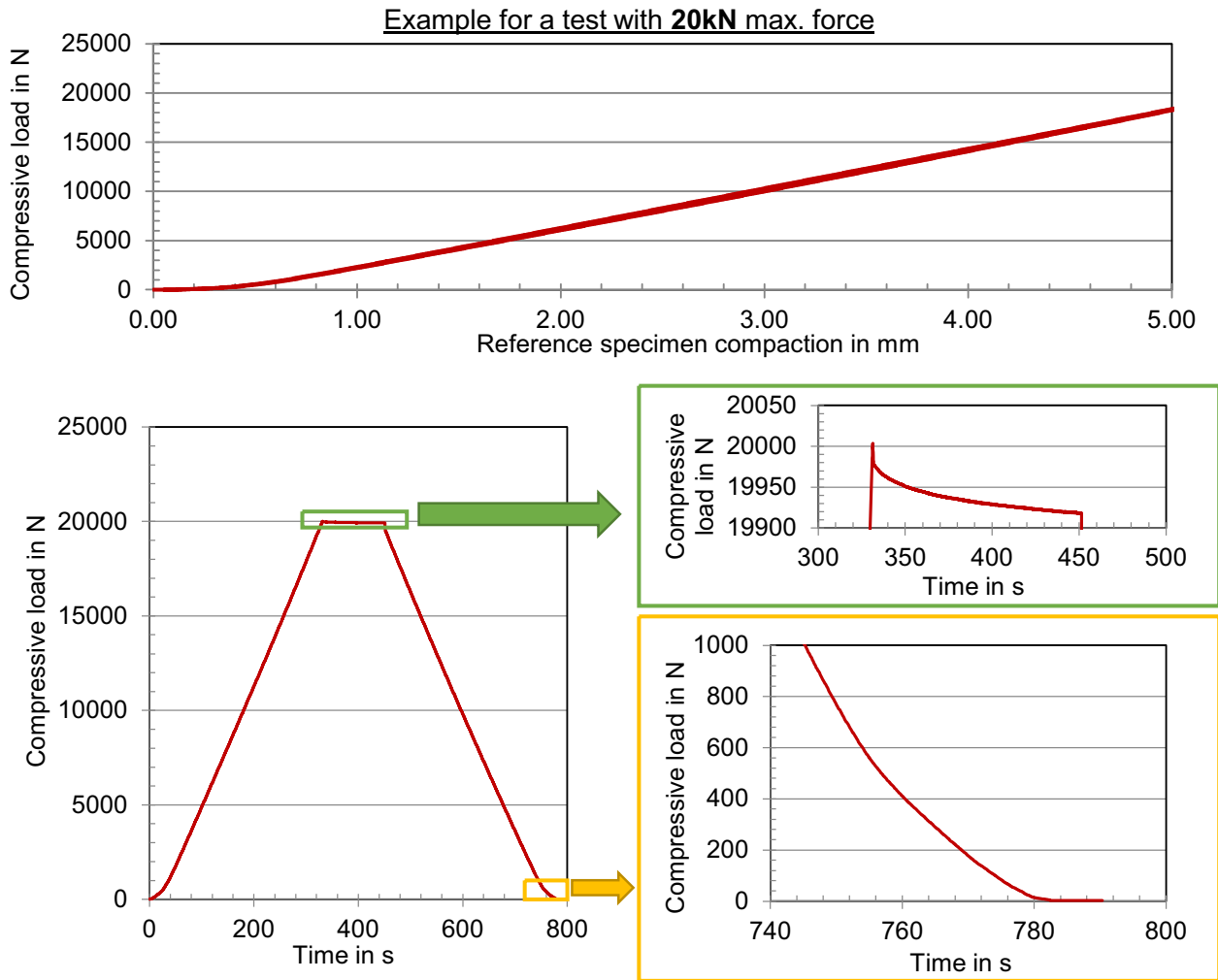
Figure 2. Exemplary compaction response of the specimen.
