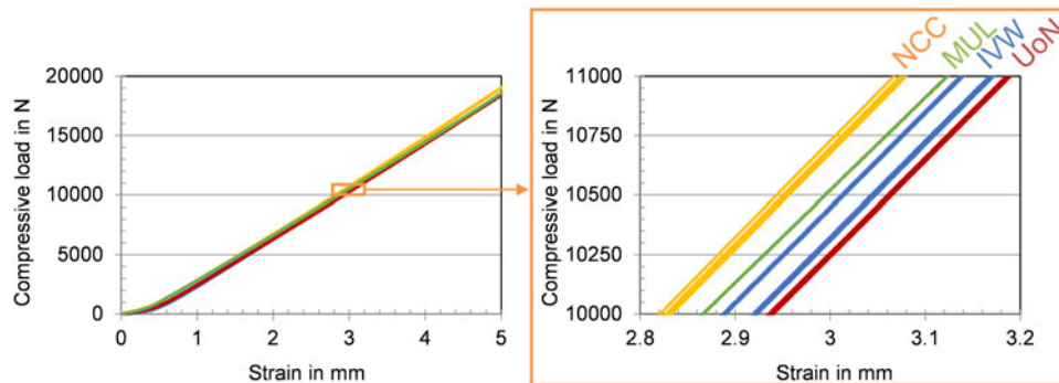
Figure 3. Comparison of the force vs. compaction curves (max. force: 20 kN) measured with the different test rigs.
