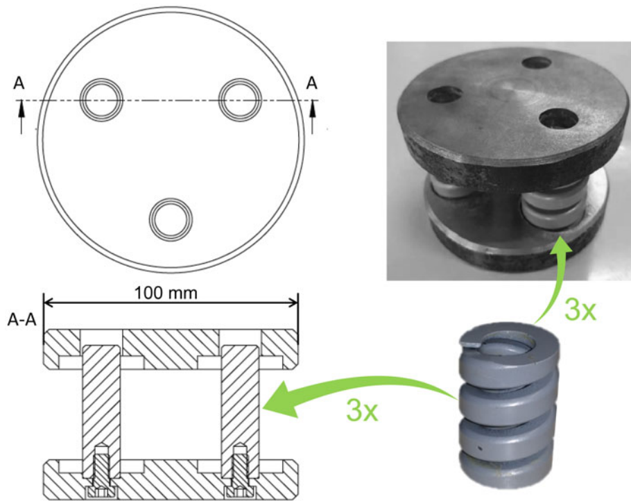
Figure 1. Technical drawing and picture of the specimen.
