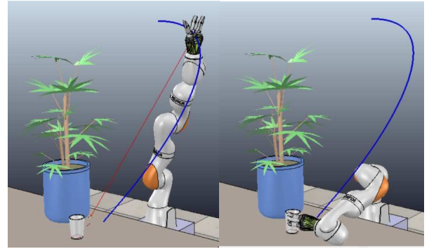
Figure 8. running time = 12.11s, total time =18.17s RRT* planning experiment on robot arm (KUKA LBR iiwa 7 R800) in V-rep, the task is to plan a route from upright state(initial position) to the cup(goal position) on the table for robot arm, the plant represents obstacle, the blue line describes the final route
