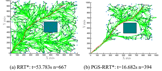
Figure 6. Near-optimal path conducted by RRT* and PGS-RRT* in a 2D space 1000*1000, the initial position is at (0, 0), the goal position at (800, 900)
