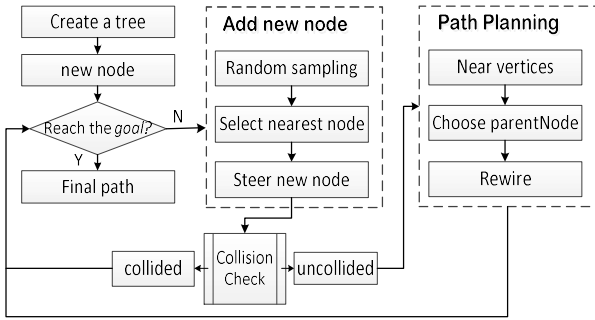
Figure 1. Program diagram of RRT*
