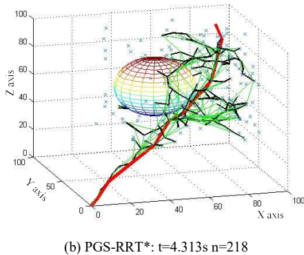
Figure 7. Near-optimal path conducted by RRT* and PGS-RRT* in a 3D space, the searching space is a square 100*100*100, the initial position is at (0, 0, 0), the goal position at (90, 90, 90), the sphere represents the obstacle, small marker 'x' represents sampling point, and the black line describes the rapidly-growing exploring tree, the green is the lower cost path after Rewire procedure, and the red path represents the final route.
