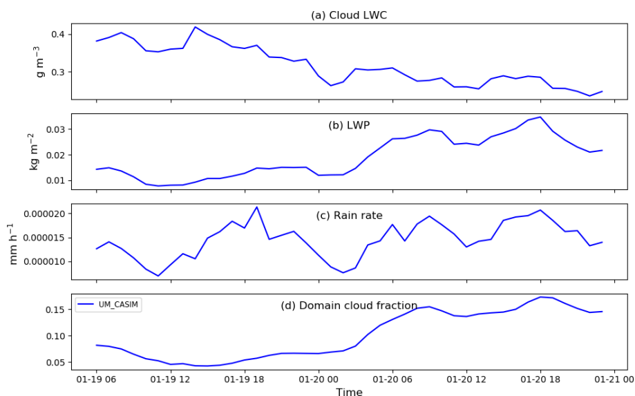
Figure 2. Time series of domain-averaged (a) cloud liquid water content (in-cloud only), (b) liquid water path, (c) rain rate, and (d) cloud fraction, all for the baseline case UM_CASIM. A liquid water content threshold of 0.01 \text{ g m}^{-3} is used to define a cloudy grid box.
