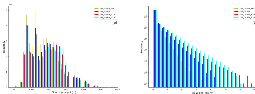
Figure 9. Histograms of cloud top height (a), calculated as the highest cloudy grid box in a cloudy column, and of total column liquid water path (b), calculated using only columns containing cloud.
