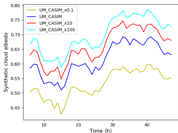
Figure 7. Time series of mean synthetic cloud albedo. This is calculated for cloudy columns only using an estimate of the cloud optical depth, as shown in Eq. (1).
