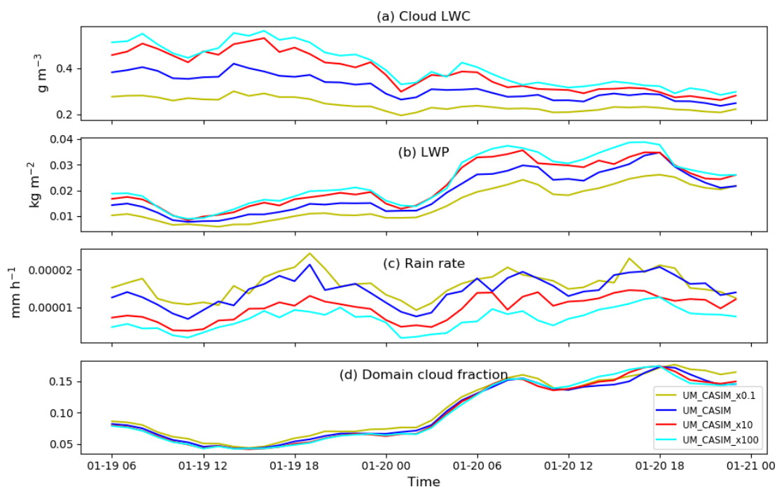
Figure 5. Time series of domain-averaged (a) cloud liquid water content (in-cloud only), (b) liquid water path (LWP), (c) rain rate, and (d) cloud fraction. A liquid water content threshold of 0.01 \text{ g m}^{-3} is used to define a cloudy grid box.
