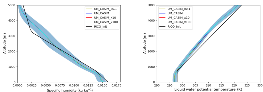
Figure 12. Average vertical profiles of liquid water potential temperature and specific humidity for each aerosol concentration, compared to the RICO initial setup as in Fig. 2, with the standard deviation of the baseline case shaded.
