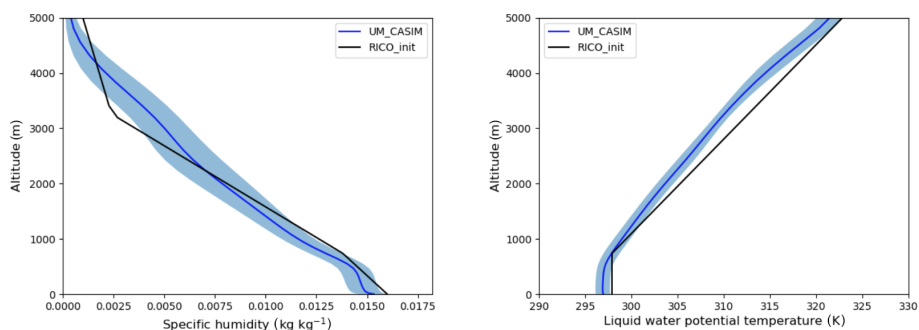
Figure 3. Domain-averaged vertical profiles of liquid water potential temperature and specific humidity for the baseline case, compared to the RICO initial setup, with the standard deviation of the baseline shaded.
