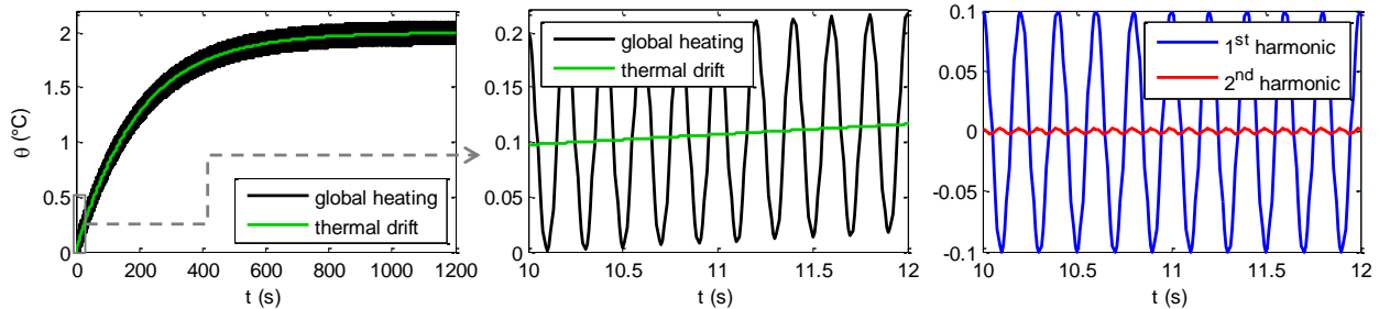
Fig. 1: Time-evolution of a simulated heating signal of a sample under cyclic loading of fixed amplitude and frequency. Global heating and thermal drift (left and middle, for a 2s time-window); first two harmonics (right).
