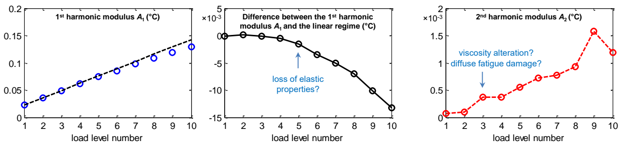
Fig. 2: Variations of the first and second harmonic moduli during a self-heating test from one load level to another (left & right). Highlight of the nonlinearity of the first harmonic (middle).
