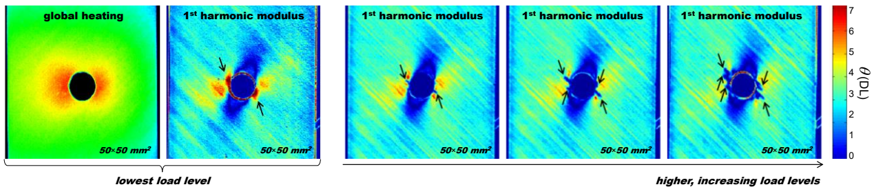
Fig. 3: Self-heating test on a carbon/epoxy UD composite with a 10 mm diameter perforation. Global heating and first harmonic modulus maps for a low load level (left); evolution of the first harmonic modulus for higher load levels (right).
