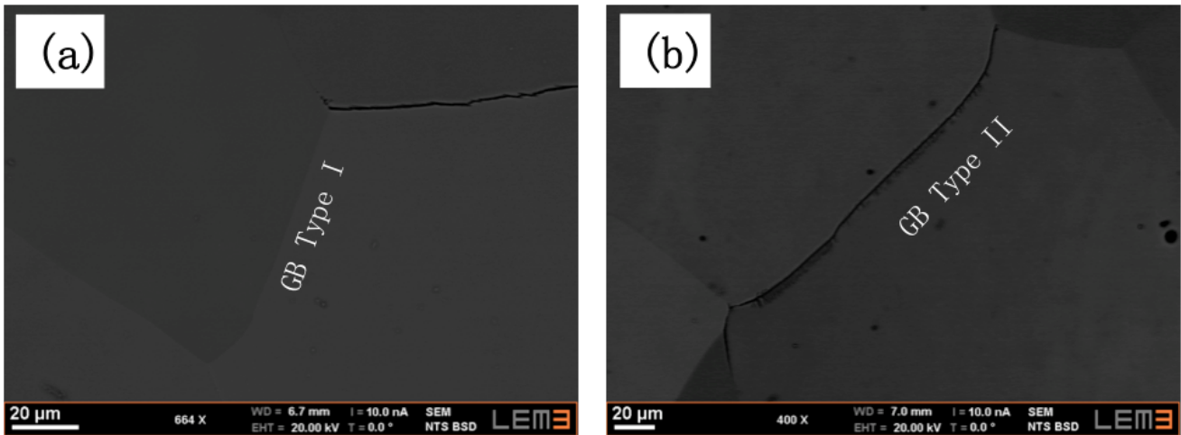
Fig.2. (a) Type I GB showing no \alpha_{GB} layer and (b) Type II GB fully decorated with an \alpha_G layer and even early emission of \alpha Widmanstätten colonies.
