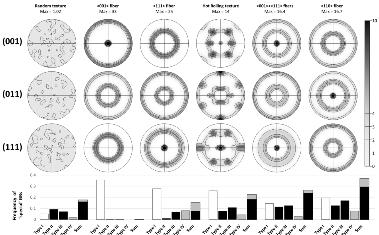
Frequency of special GBs for typical textures according to the Monte-Carlo approach.
