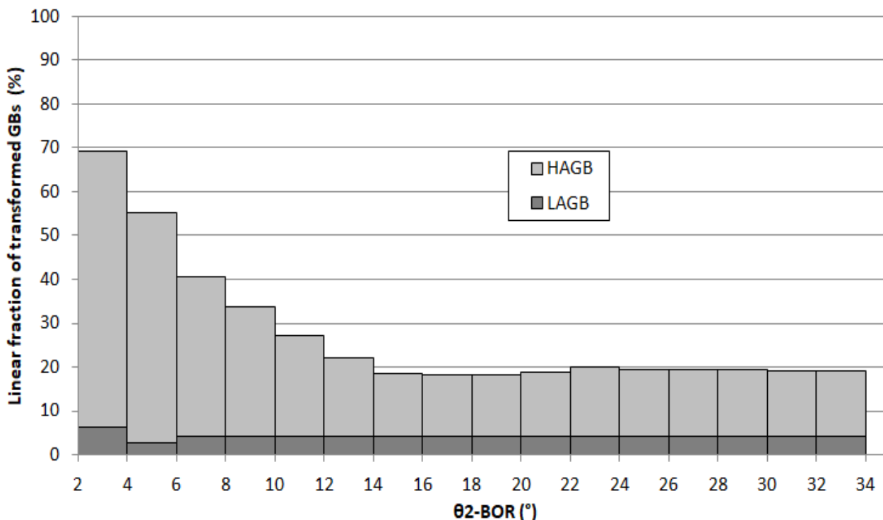
Fig. 1. Fraction of transformed boundaries as a function the disorientation to the closest ‘special’ boundary.
