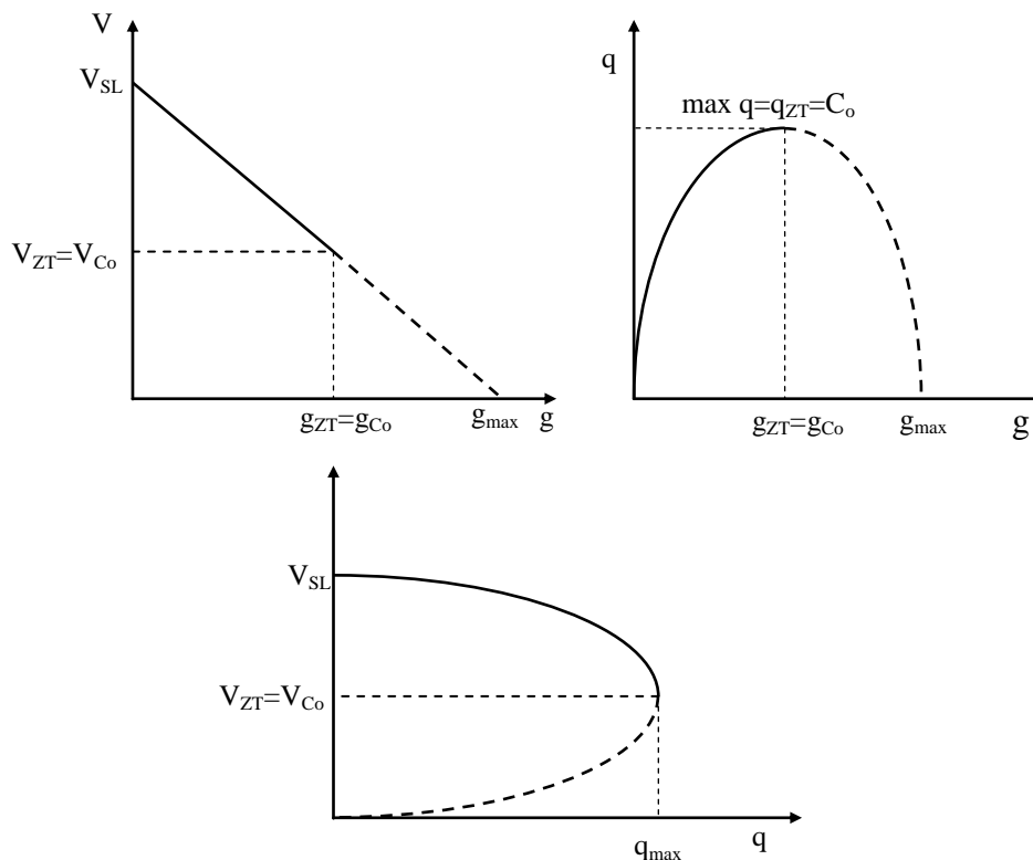
Fig. 1. Graphic presentation of the generalized relationship among the speed, density and flow rate, in theoretical ideal conditions
