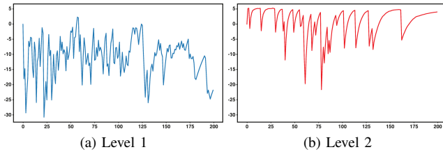
Fig. 6: Level 1 vs level 2 average welfare, from Importance Sampling estimation.
