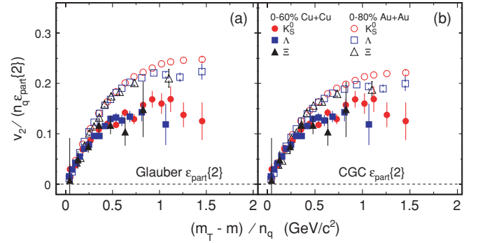
FIG. 14. (Color online) Number of quarks and participant eccentricity scaled v_2 [ v_2 / (n_q \epsilon_{\text{part}}\{2\}) ] of identified particles as a function of (m_T - m) / n_q in 0%–80% Au + Au collisions (open symbols) [31] and 0%–60% Cu + Cu collisions (solid symbols) at \sqrt{s_{NN}} = 200 GeV. Circles, squares, and triangles represent the data for K_S^0 , \Lambda , and \Xi , respectively. The error bars are shown only for the statistical uncertainties.
