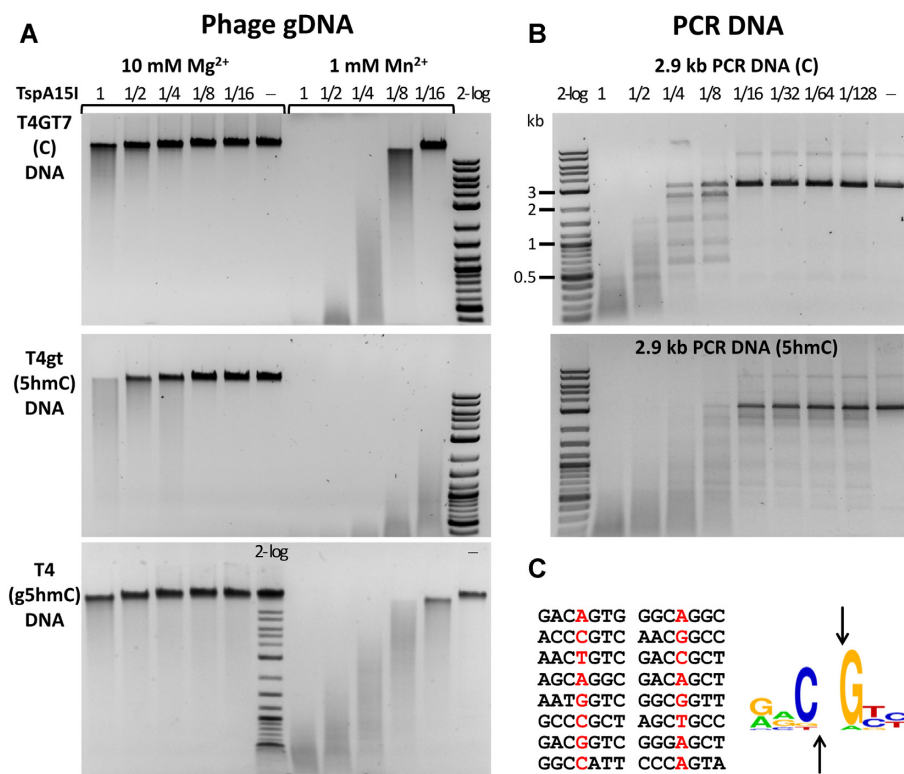
Figure 3. TspA15I restriction activity in vitro . (A) TspA15I digestion of phage T4GT7 (unmodified C), T4gt (5hmC) and WT T4 (g5hmC) gDNAs. Digestions were carried out in 10 mM Mg^{2+} or 1 mM Mn^{2+} buffer. (B) TspA15I digestion of C- and 5hmC-containing PCR DNA. 0.5 \mu g of PCR DNA ( \sim 5.3 nM) was incubated with TspA15I enzyme in 2-fold serial dilutions, starting at 1 \mu g (280 nM) for 1 h in Mn^{2+} buffer. At 1/16 to 1/128 dilutions ( \sim 17.5 nM to 2.2 nM range) the enzyme cleaves modified DNA more efficiently. The 2 log DNA ladder (2-log, 0.1 to 10 kb) was used for size marker in all presented digestions. (C) Mapping of cut/nick sites. The cut/nick sites were sequenced from 5hmC-modified PCR DNA digested by TspA15I in Mn^{2+} buffer (the base before the cut site is marked in red) and the 5hmCNG logo was generated with WebLogo (27).
