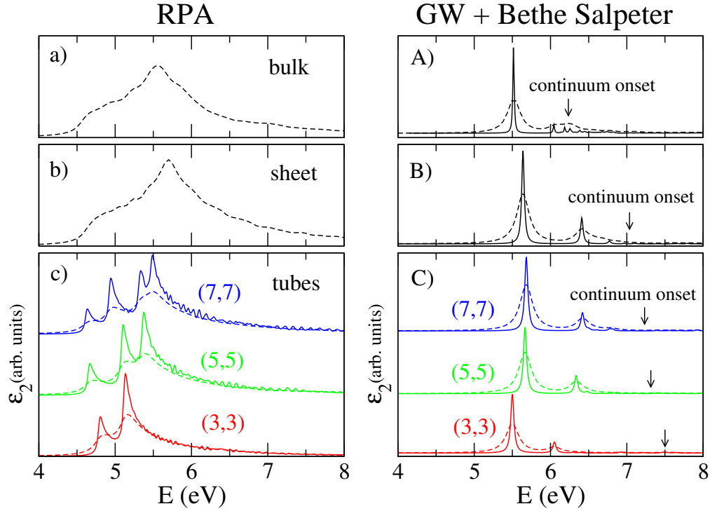
FIGURE 2. Optical absorption of hBN (a), BN-sheet (b) and three different BN tubes (c). We compare the results of the GW + Bethe-Salpeter approach (right hand side) with the random phase approximation (left hand side). Solid lines are calculated with a Lorentzian broadening of 0.025 eV, dashed lines with a broadening of 0.1 eV (for comparison with experimental data). The light polarization is parallel to the plane/ tube axis, respectively.
