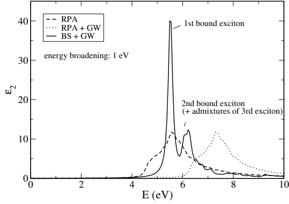
FIGURE 1. Optical absorption of bulk hBN calculated on three levels of approximation (see text).
