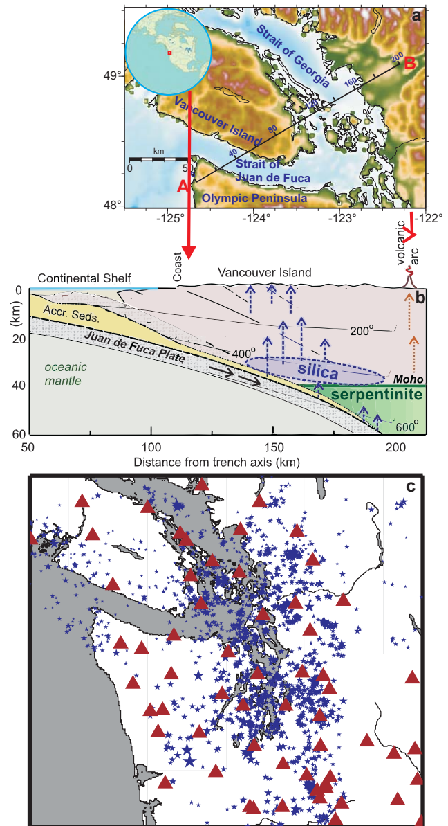
Fig. 1. (a) Location map of the study region. Distance along the profile is marked in kilometers. (b) schematic along line AB showing the subduction zone structure. (c) map view of stations and earthquakes used in tomography. Vertical cross-sections of P- and S-wave velocity along profile AB are shown in Fig. 4.
