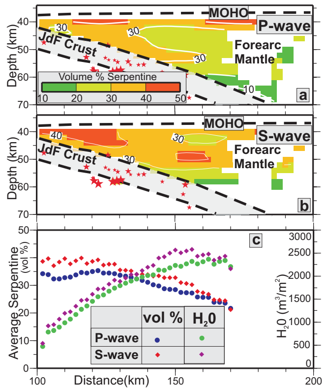
Fig. 6. Plot of volume percent serpentinization in the forearc mantle computed from (a) P-wave velocity and (b) S-wave velocity for the region enclosed by the red box in Fig. 4c (100–200 km distance on profile AB shown in Fig. 1). (c) Plot of average volume % serpentine and total water content in a unit column of the forearc mantle.
