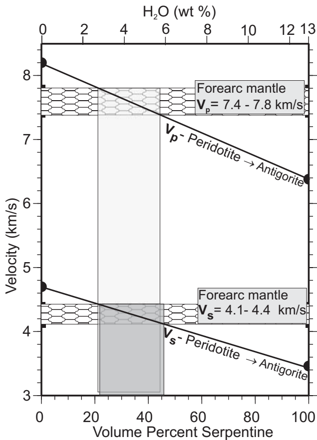
Fig. 5. Plot of peridotite-antigorite assemblage velocity versus volume percent serpentinization (velocity of antigorite taken from (Christensen, 2004)). The observed range of P- and S-wave velocity is shown by the hatched region. The vertical shaded regions show the volume serpentinization corresponding to the observed P and S velocity range.
