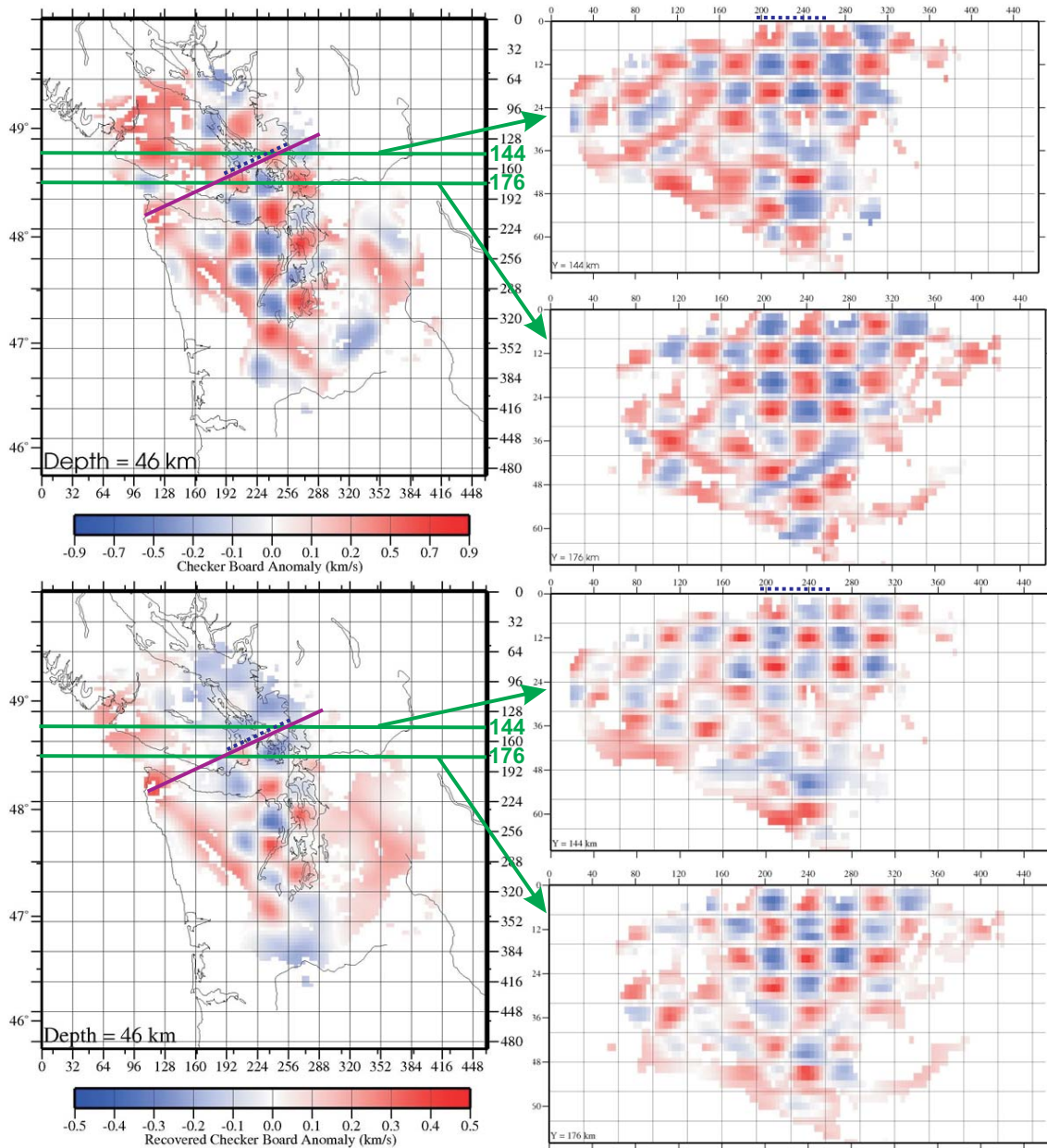
Fig. 3. Recovered P-wave (top) and S-wave (bottom) checkerboard anomaly pattern ( 32 \text{ km} \times 32 \text{ km} \times 8 \text{ km} ) for estimating horizontal and vertical resolution is shown in the figure by one horizontal slice at 46 km depth (shown on the left) and two E–W vertical slices (close to the main profile) at distances of 144 km and 176 km positions in the N–S direction (shown on the right). Purple line marks the position of the main cross-section discussed in the main article. Blue dotted line shows the inferred position of the forearc mantle wedge.
