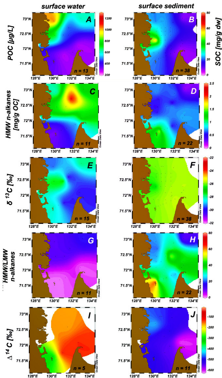
Fig. 2. Spatial distribution of organic carbon concentrations and characteristics possibly diagnostic of sources in the Buor-Khaya surface water particles (left column) and surface sediment (right column) in August 2008. n refers to the number of stations the parameter extrapolation is based upon. (A) particulate organic carbon, (POC) ( \mu\text{g l}^{-1} ); (B) surface sediment organic carbon (SOC) ( \text{mg g}^{-1} \text{ dw} ); (C) and (D) the sum of high molecular weight (HMW) n -alkanes, i.e. the sum of chain lengths \text{C}_{20}\text{--C}_{34} in POC and SOC, respectively ( \text{mg g}^{-1} \text{ OC} ); (E) \delta^{13}\text{C}_{\text{SOC}} (‰); (F) \delta^{13}\text{C}_{\text{POC}} (‰); (G) and (H) HMW/LMW n -alkanes, where LMW is low molecular weight, i.e. sum of \text{C}_{17}\text{--C}_{19} in POC and SOC, respectively; (I) \Delta^{14}\text{C}_{\text{POC}} (‰); (J) \Delta^{14}\text{C}_{\text{SOC}} (‰).
