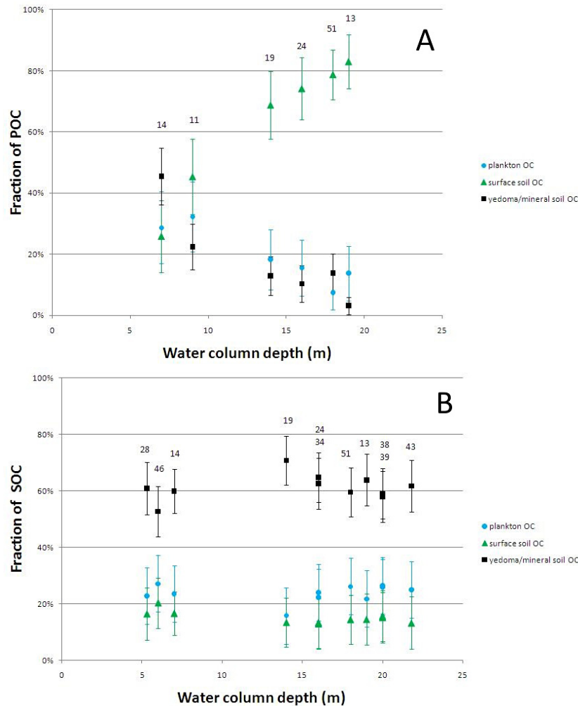
Fig. 4. Results of three end-member mixing model (Monte Carlo simulation) analysis of relative contributions from marine plankton ( f_{\text{plankton}} ; blue circles), surface soil ( f_{\text{surfsoil}} ; green triangles) and old yedoma/mineral soil ( f_{\text{yedoma/mineral soil}} ; black squares) to (A) surface water particulate organic carbon (POC) and (B) surface sediment organic carbon (SOC) in Buor-Khaya Bay in August 2008.
