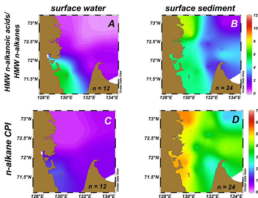
Fig. 5. Spatial distribution of organic matter degradation proxies in the Buor-Khaya Bay surface water and surface sediment in August 2008. (A) and (B) high molecular weight (HMW) i.e. the sum of chain lengths \text{C}_{20}\text{--}\text{C}_{34} n -alkanoic acids over HMW n -alkanes in POC and SOC, respectively; (C) and (D) n -alkane carbon preference index (CPI), i.e. calculated as \frac{1}{2} \sum (X_i + X_{i+2} + \dots + X_n) / \sum (X_{i-1} + X_{i+1} + \dots + X_{n-1}) + \frac{1}{2} \sum (X_i + X_{i+2} + \dots + X_n) / \sum (X_{i+1} + X_{i+3} + \dots + X_{n+1}) , where X is concentration.
