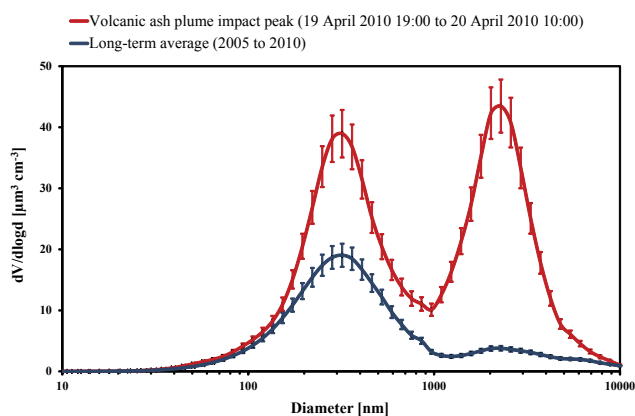
Fig. 3. Hourly average particle volume size distributions during the volcanic ash plume impact in comparison to the long-term average of the years 2005 to 2010 at the University of Applied Sciences in Augsburg, Germany. The error bars represent \pm 10\% .
