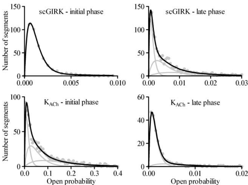
FIGURE 13 Modal distributions of scGIRK and K_{ACh} channels associated with the opposing regulation of these channels. Open probability histograms generated from the homogeneous phases of scGIRK ( top panels ) and K_{ACh} ( bottom panels ) channel gating shown in Fig. 12. For the scGIRK channel the mean p_o values and relative areas (given in parentheses) of different components are p_{o1} = 0.00060 (87.2%) and p_{o2} = 0.0030 (12.8%) for the initial phase; and p_{o1} = 0.00061 (34.3%), p_{o2} = 0.0026 (40.3%), and p_{o3} = 0.0072 (25.4%) for the late phase of channel activation. For the K_{ACh} channel the mean p_o values and the relative areas of different components are p_{o1} = 0.0073 (26.3%), p_{o2} = 0.0268 (40.0%), and p_{o3} = 0.0780 (33.7%) for the initial phase; and p_{o1} = 0.00068 (79.4%), p_{o2} = 0.0032 (18.7%), and p_{o3} = 0.0080 (1.9%) for the late phase of channel activation. The P values, determined from these distributions, are P^{initial} = 0.084 and P^{late} = 0.440 for the scGIRK channel; and P^{initial} = 0.503 , and P^{late} = 0.130 for the K_{ACh} channel. The K_{ACh} channel gating during the late phase is impaired not only by its confinement within the low-efficient modes 1 and 2, but also by the significant reduction in the open probability of individual kinetic components contributing to channel activity.
