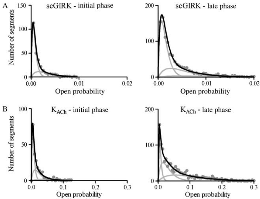
modes. (B) Open probability histograms generated from the initial (left panel) and late (right panel) phases of K ACh channel activity shown in Fig. 9. The mean p_o values and the relative areas of different components are p_{o1} = 0.0033 (50.0%), p_{o2} = 0.012 (37.5%), and p_{o3} = 0.031 (12.5%) for the initial phase; and p_{o1} = 0.0033 (20.3%), p_{o2} = 0.015 (37.4%), and p_{o3} = 0.053 (42.3%) for the late phase of channel activation. The P values computed from these histograms are P^{\text{initial}} = 0.328 and P^{\text{late}} = 0.555 for the K ACh channel. Thus, the changes in the gating behavior for this K ACh channel were mostly associated with a shift in the modal equilibrium toward gating modes 3 and 4.
