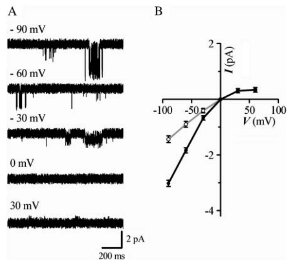
FIGURE 3 Voltage dependence of scGIRK and K_{ACh} channels. (A) G\beta_1\gamma_7 -activated single-channel currents were recorded from the same membrane patch at the indicated potentials. All-points histograms were generated from the recordings and fitted by a sum of Gaussian functions to determine the mean current amplitudes. (B) I-V curves for the scGIRK (gray) and K_{ACh} (black) channels were constructed from the single-channel current amplitudes determined at each membrane potential. Each data point represents the mean \pm SEM of currents recorded from 5 to 14 channels.
