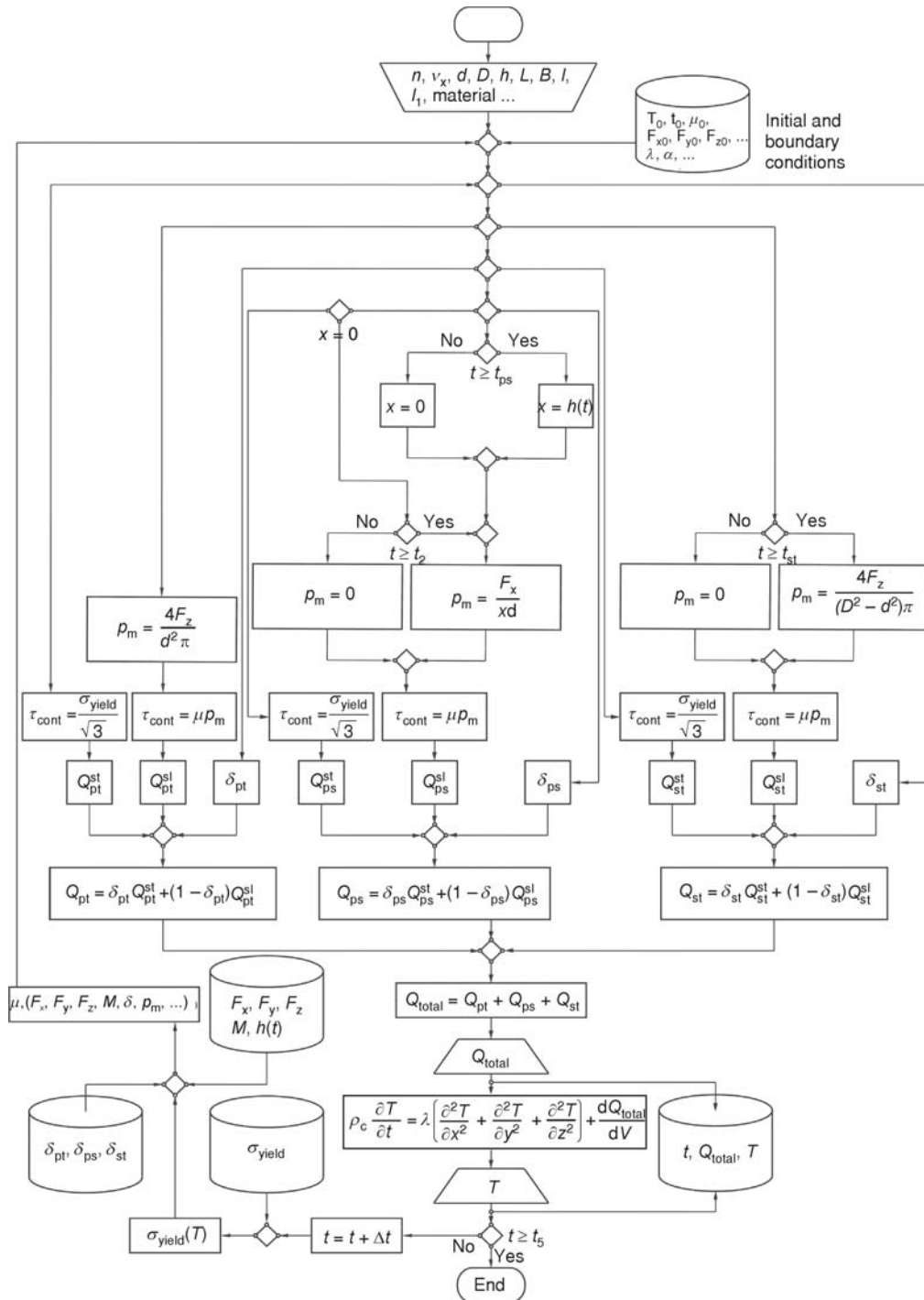
Figure 5. Flow chart of an algorithm software
