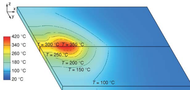
Figure 6. Numerical certain temperature field work pieces, a moment t = 40.6285 \text{ s} , maximum temperature T_{\text{max}} = 393.538 \text{ °C} at the point with co-ordinates (x, y, z) = (30.5, 53, 4)
