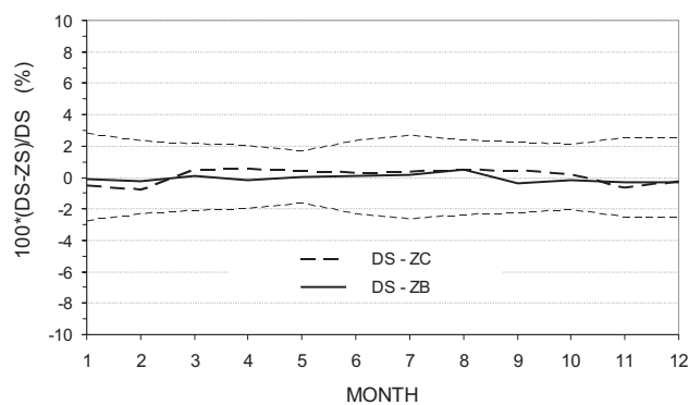
Fig. 1. Monthly average relative differences and their 1-STD limits between simultaneous Dobson and Brewer DS , ZB and ZC total ozone observations, Hradec Kralove, 1994–2004, updated seasonal zenith polynomials.
