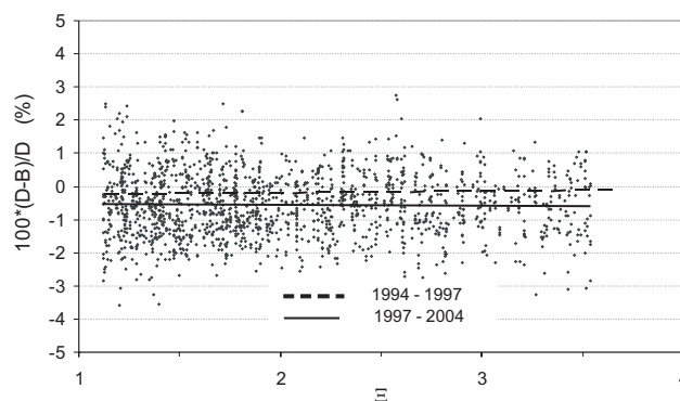
Fig. 3. Linear approximations of relative differences between simultaneous Dobson and Brewer Direct Sun total ozone observations – corrected data sorted by relative optical air masses of the ozone layer Hradec Kralove, 1994–2004.
