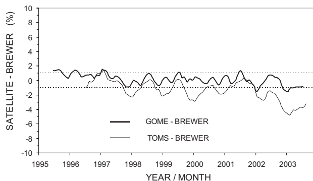
Fig. 6. Relative differences between simultaneous satellite and Brewer DS total ozone observations and 1-percent precision limits, Hradec Kralove, July 1995–June 2003.
