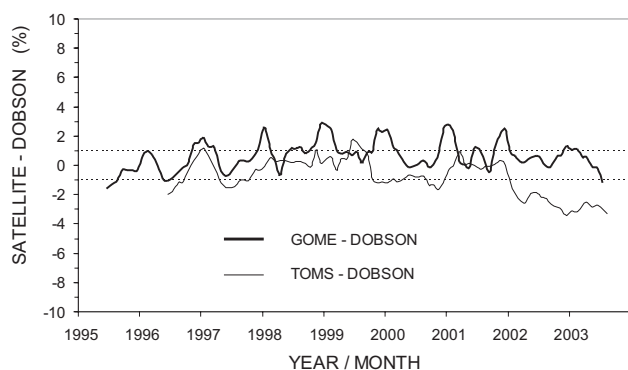
Fig. 5. Relative differences between simultaneous satellite and Dobson DS total ozone observations and 1-percent precision limits of the Dobson spectrophotometer, Hradec Kralove, July 1995–June 2003.
