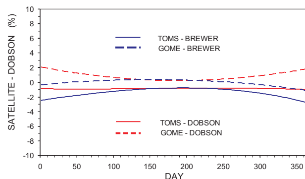
Fig. 7. Smoothed annual course of relative differences between simultaneous satellite and ground DS total ozone observations, Hradec Kralove, July 1996–June 2003.
