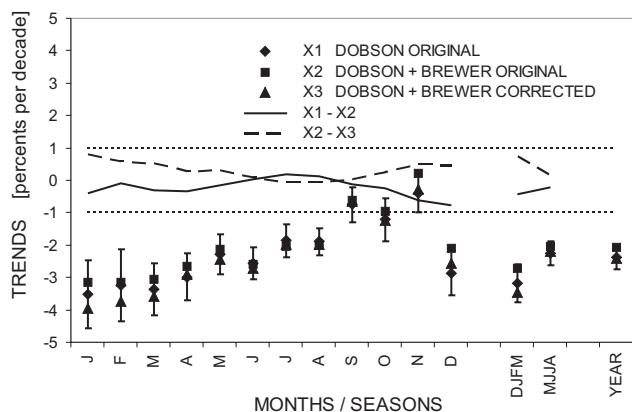
Fig. 4. Monthly and seasonal trends of the re-evaluated X1, combined X2 and corrected-combined X3 and differences between trends X1-X2, X2-X3 of Dobson and Brewer total ozone data series, Hradec Kralove, 1967–2004.
