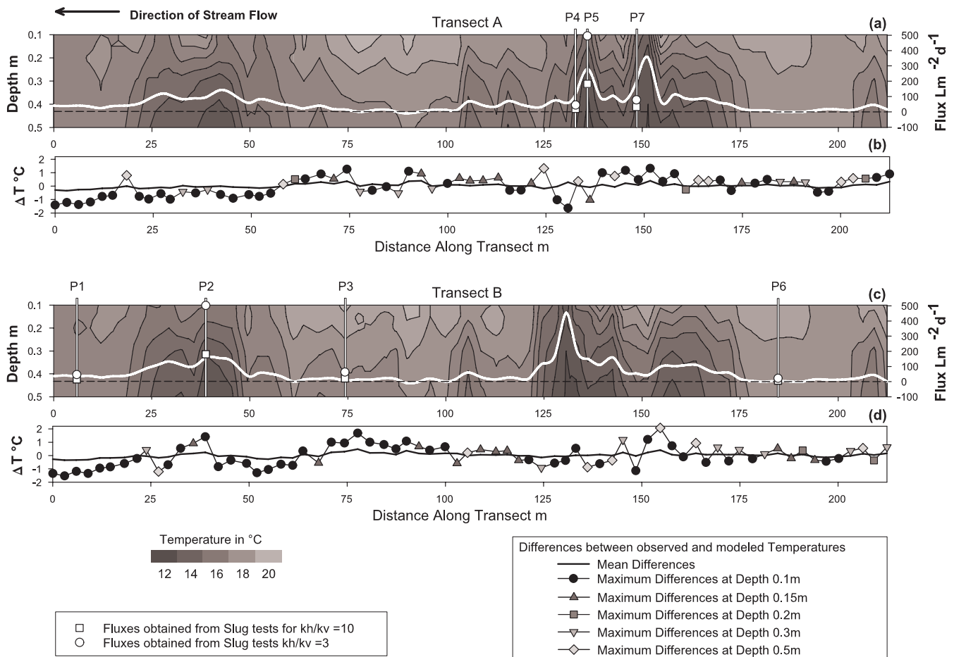
Fig. 4. Temperature distribution, temperature based fluxes, the locations of streambed piezometers, and the fluxes from Darcy’s law calculations at each piezometer for different anisotropy ratios along Transects A (a) and B (c). Note the vertical exaggeration of the longitudinal profile by factor 50.
