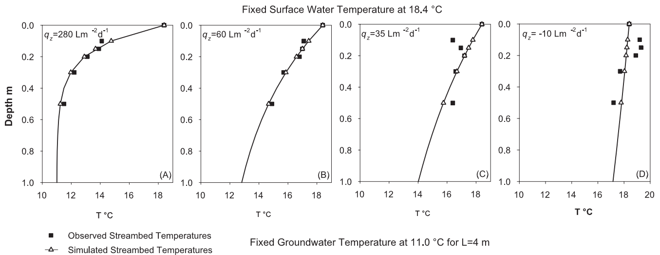
Fig. 7. Comparison of observed and simulated streambed temperatures for four example profiles. The illustrated profiles represent high (a), medium (b), low (c) groundwater discharges and low recharge conditions (d). The profiles are located proximal to the positions of streambed piezometers P5 (a), P4 (b), P1 (c) and P3 (d).
