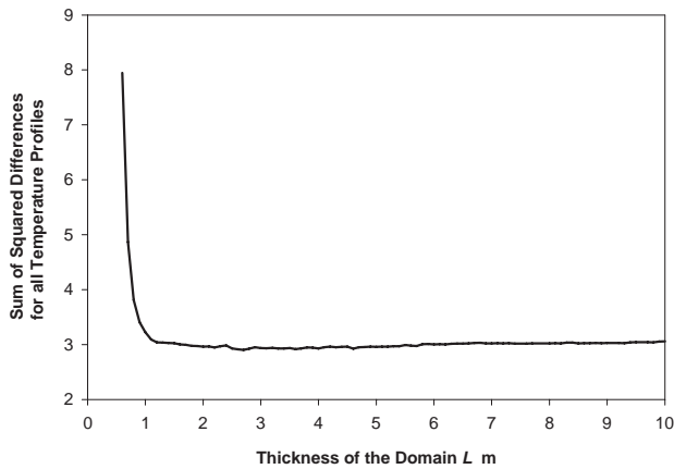
Fig. 5. Sum of squared errors of all temperature profiles vs. the thickness of the domain L . The results show that for the given parameter set, the quality of fit and the derived vertical fluxes are essentially constant for L > 1.0 m.
