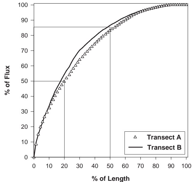
Fig. 6. Percentage of flux vs. percentage of length of the Transects A and B. Approximately 50% of the total flux occur on 20% of the total length.
