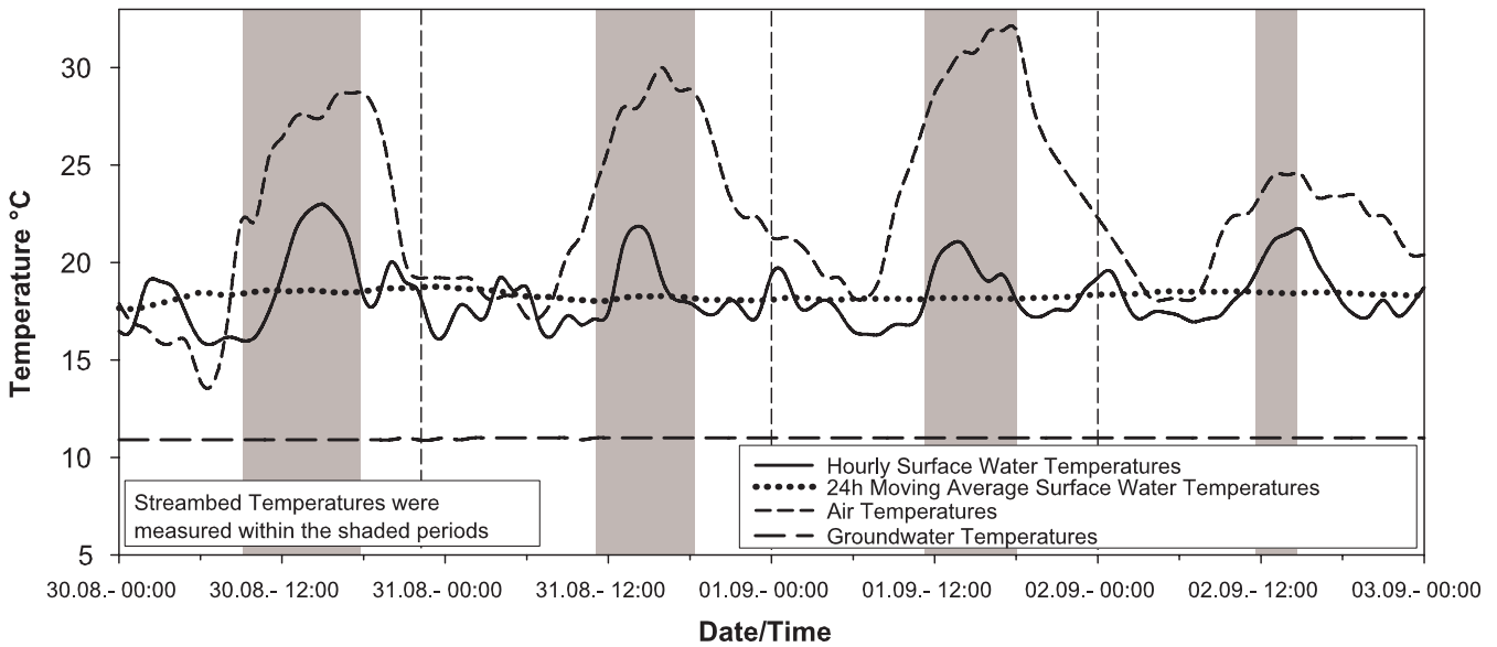
Fig. 3. Surface water, air and groundwater temperatures during the four day measurement programme in August/September 2005.
