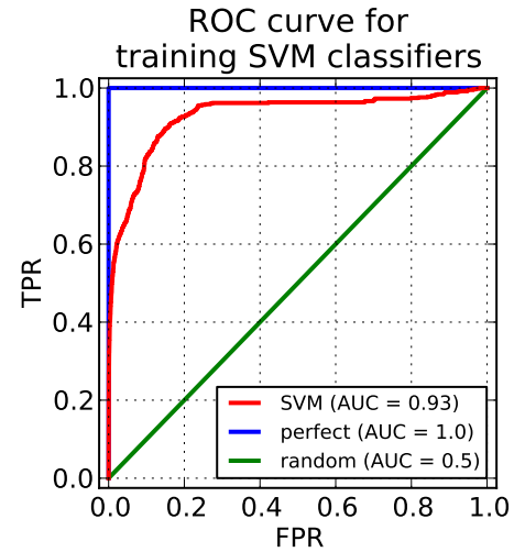
Fig. 6. Receiver operating characteristic for the bootstrapped set of individual SVM classifiers assessed using holdout test data. SVM training parameters ( \gamma = 0.1 , C = 3 ) are chosen to maximize the area under the ROC curve.
