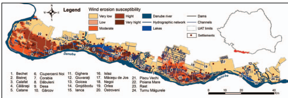
Fig. 5 Wind erosion susceptibility of the Danube Floodplain, Calafat-Turnu Măgurele sector
