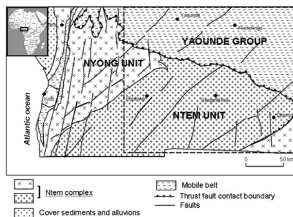
Figure 1 Schematic map of the south-western Cameroon. The Ntem complex consists of the Ntem and Nyong units. The study area is marked with dotted lines.
