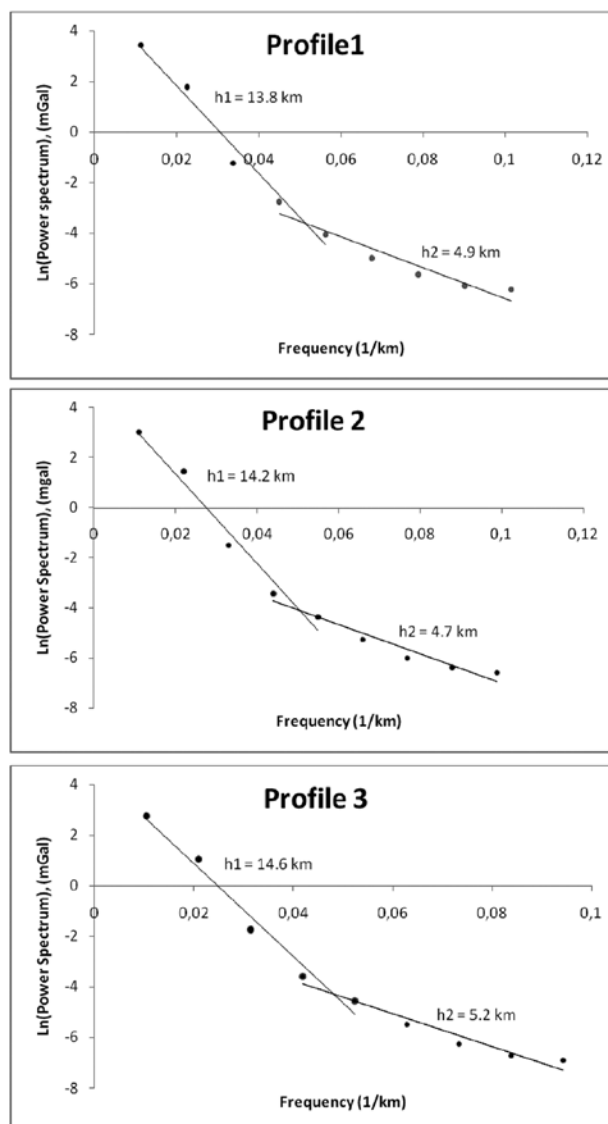
Figure 7 Plots of power spectrum versus the frequency for profiles P1, P2 and P3. h1: deep density contrast plane; h2: shallow density contrast plane
