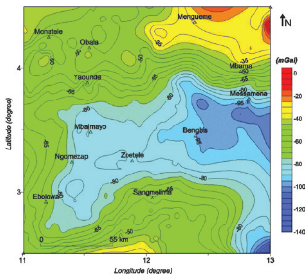
Figure 4 Bouguer anomaly map of the study area.
