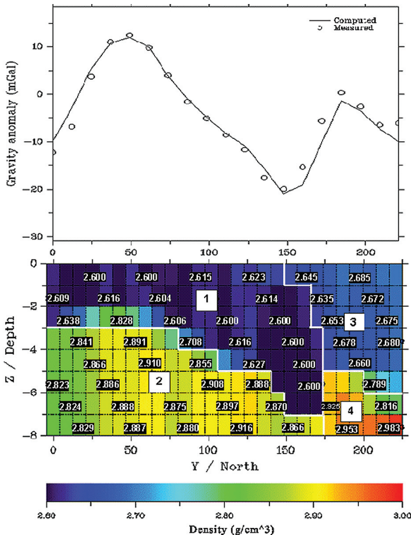
Figure 9 3D density model cross section (S2). 1: So'o granites; 2: Charnockites; 3: Pan-African formations; 4: Deep structures in Pan-African belt (granulites). In the upper box are shown the measured and calculated gravity anomalies.
