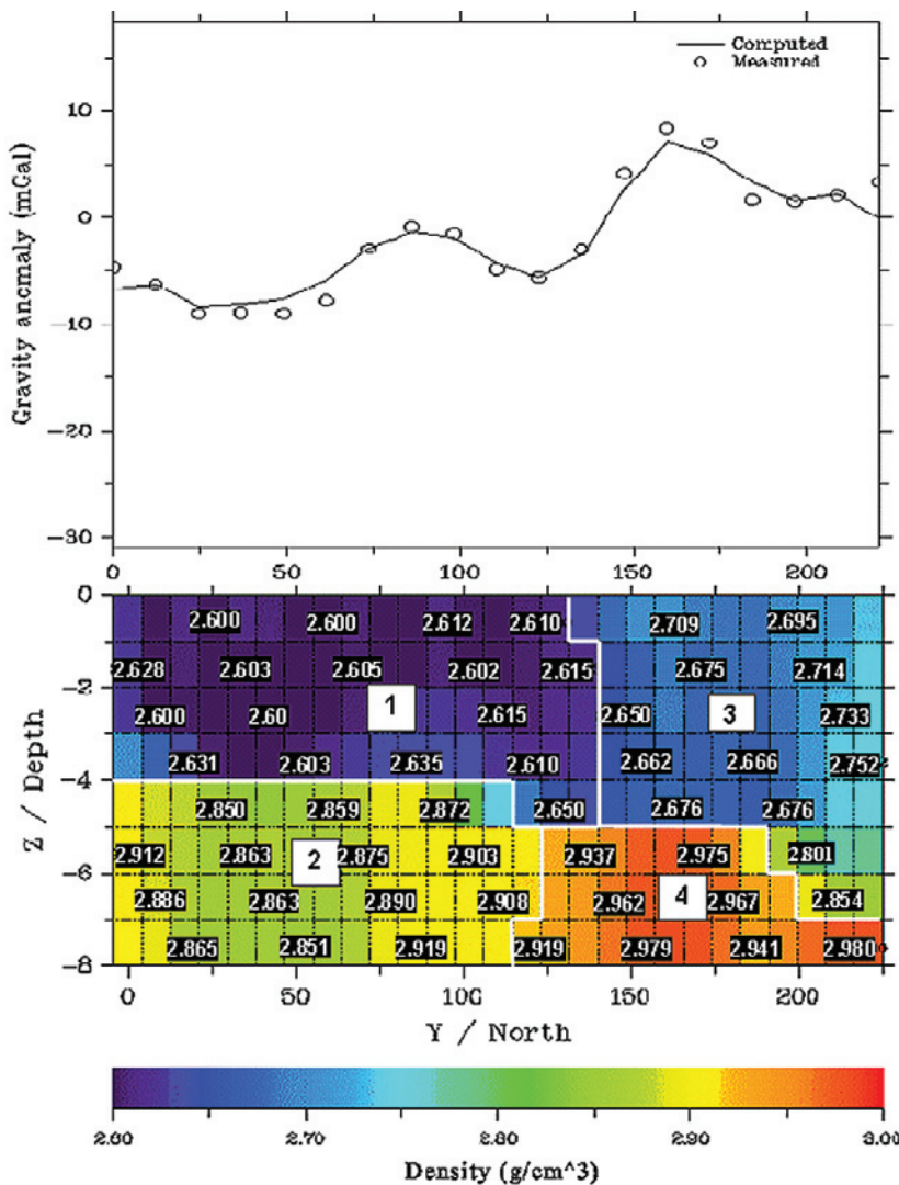
Figure 8 3D density model cross section (S1). 1: So'o granites; 2: Charnockites; 3: Pan-African formations; 4: Deep structures in Pan-African belt (granulites). In the upper box are shown the measured and calculated gravity anomalies.
