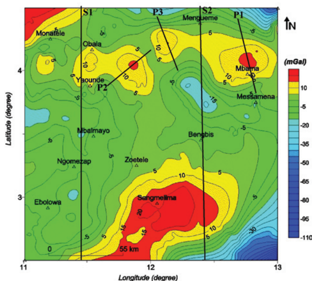
Figure 6 Third-order residual anomaly map of the study area (Intervals : 5 mGal) showing studied profiles (P1, P2 and P3) and selected 3-D density model cross sections (S1 and S2).
