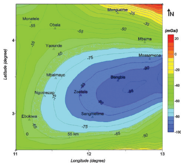
Figure 5 Third-order regional anomaly map of the study area.
