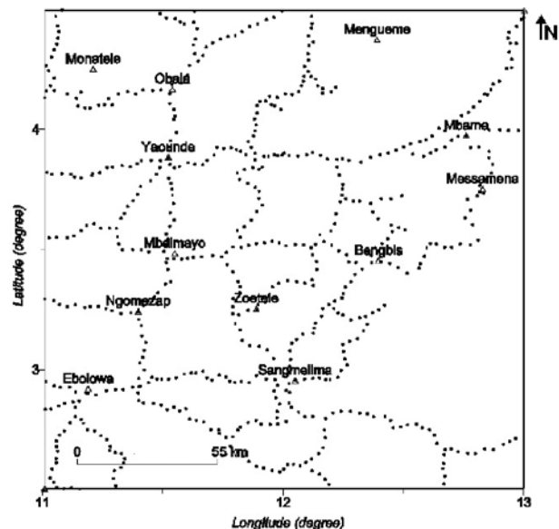
Figure 3 Study area map showing the gravity stations (dots).
