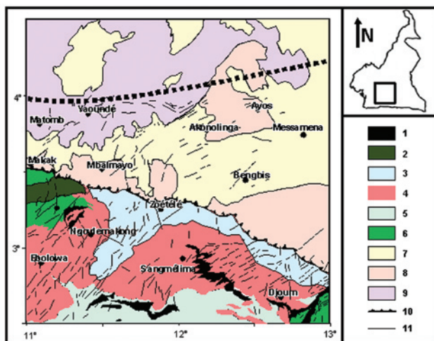
Figure 2 Geological sketch map of the study area (after Maurizot, 2000). 1. Iron formation; 2. Orthopyroxène bearing gneiss; 3. Tonalitic suite (TTG); 4. Charnockitic suite (TTG); 5. Banded series; 6. Biotite-horblende gneiss; 7. Micashists (YS); 8. Epischist (MB); 9. Gneiss (YS); 10. Major thrust (Pan African); 11. Lineaments. The dashed line at the latitude of Yaoundé (4°N) is the assumed limit of the Congo craton (this study).
