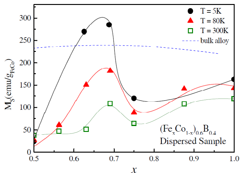
Figure 7. Saturation magnetization vs. composition for (\text{Fe}_x\text{Co}_{1-x})_{0.6}\text{B}_{0.4} dispersed nanoparticles at T = 5 K, 80K, and 300 K. The dashed line is the M_S bulk alloy value from [1]. The solid lines are only a guide to the eye.
