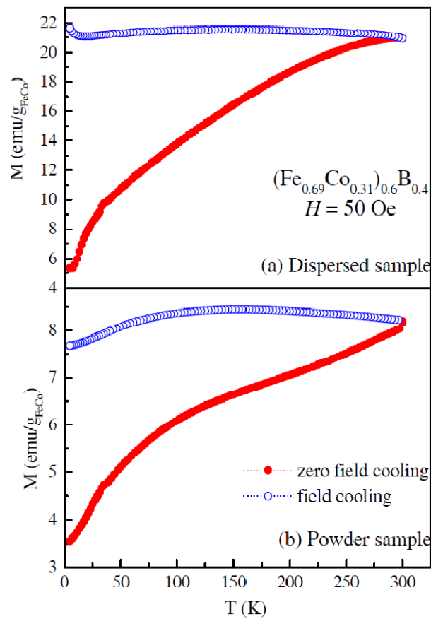
Figure 2. Magnetization vs. temperature curves for (\text{Fe}_{0.69}\text{Co}_{0.31})\text{B}_{0.4} dispersed (a) and powder (b) particles measured under zero-field-cooling (ZFC) and field-cooling (FC) conditions.
