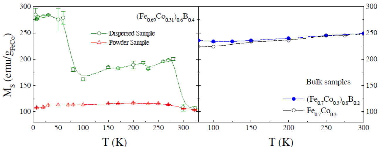
Figure 5. Saturation magnetization ( M_S ) vs. temperature for dispersed (non-interacting) and powder (with strong interparticle interactions) (\text{Fe}_{0.69}\text{Co}_{0.31})\text{B}_{0.4} particles, and the bulk (\text{Fe}_{0.7}\text{Co}_{0.3})_{0.8}\text{B}_{0.2} and \text{Fe}_{0.7}\text{Co}_{0.3} samples. The lines are only a guide for the eye.
