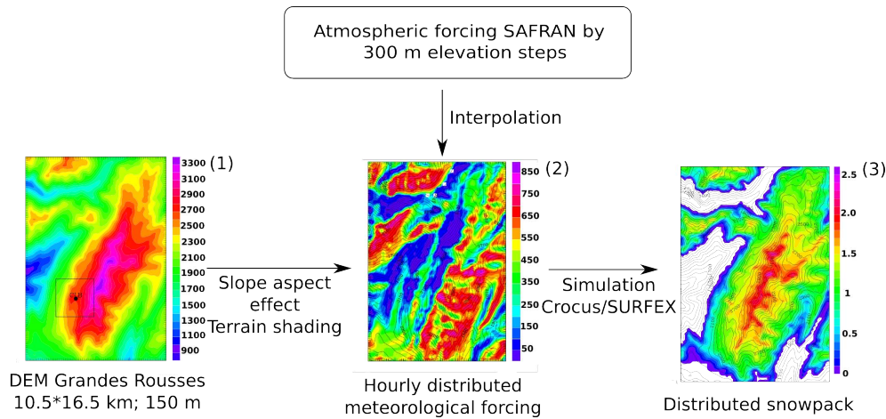
Fig. 7. Flow chart of the distributed simulation over the Grandes Rousses range. (1) DEM Grandes Rousses (150 m) (2) Incoming shortwave radiation (diffuse+direct, W m^{-2} ) on 2011/02/18 10:00 (3) Snow depth (m) on 2011/04/15 06:00.
