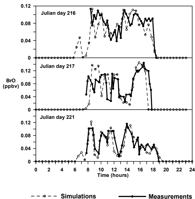
Fig. 5. Comparison between measured and simulated BrO. This graph presents only measurements of BrO concentrations above 20 pptv.
