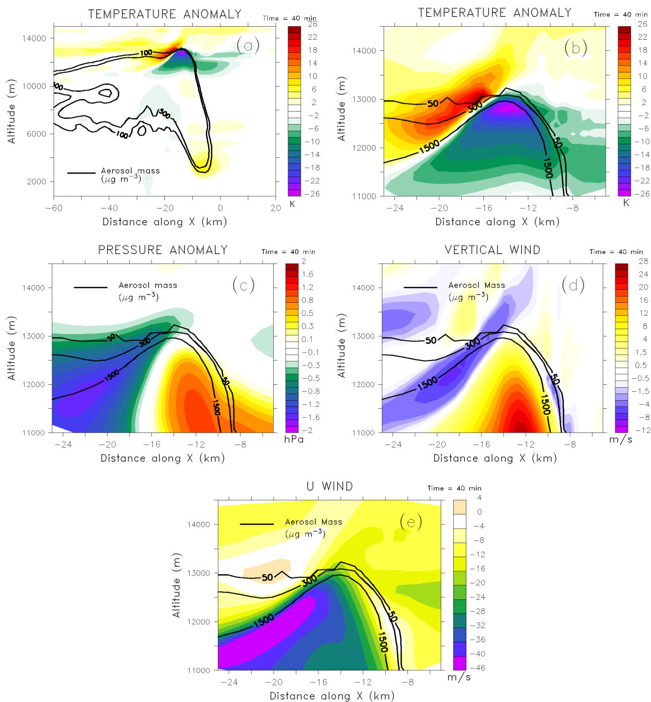
Fig. 8. Vertical cross-sections of (a, b) temperature anomaly, (c) pressure anomaly, (d) vertical wind field, and (e) u -component of the horizontal wind at y = -5 km. Solid black lines indicate isolines of aerosol concentration. Temperature and pressure anomalies are defined as the difference with respect to the background temperature and pressure profiles. The distinct bipolar structure is a clear indication of gravity wave activity.
