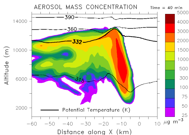
Fig. 4. Aerosol mass concentration along the y=-5 \text{ km} vertical cross section after 40 min. Contour lines indicate potential temperature levels. The tropopause was located at \theta=332 \text{ K} .
