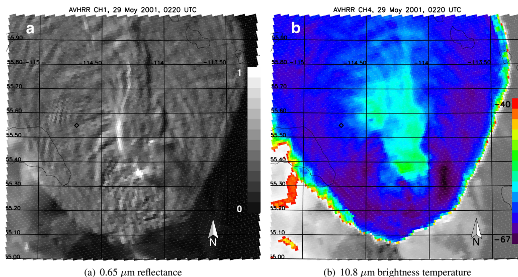
Fig. 1. Images from a NOAA AVHRR overpass during the mature phase of pyroCb convection. Reflectance in the visible 0.65\ \mu\text{m} channel is depicted in (a), brightness temperatures measured by the 10.8\ \mu\text{m} thermal IR channel are shown in (b). Reproduced from Rosenfeld et al. (2007).
