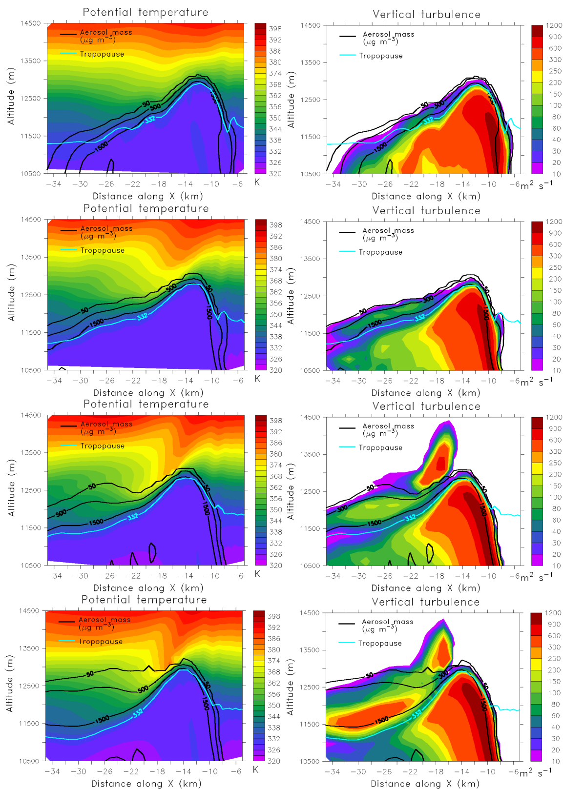
Fig. 9. Vertical cross sections of potential temperature (left column) and vertical turbulent exchange coefficient (right column) for four different points in time. Due to the anisotropic treatment of turbulence in ATHAM (Herzog et al., 2003), the vertical turbulent exchange coefficient K_{\text{ver}} is related to the horizontal turbulent exchange coefficient K_{\text{hor}} as K_{\text{ver}} = \frac{1}{\sqrt{2}} K_{\text{hor}} .
