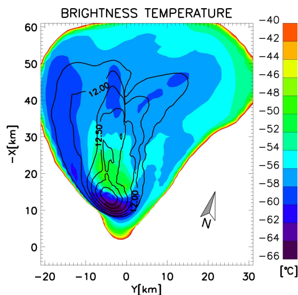
Fig. 7. Brightness temperatures derived from upwelling radiance simulated for the 10.8 \mu\text{m} wavelength band. The contour lines indicate the altitude in km of the 100 \mu\text{g m}^{-3} isosurface of the aerosol mass concentration.
