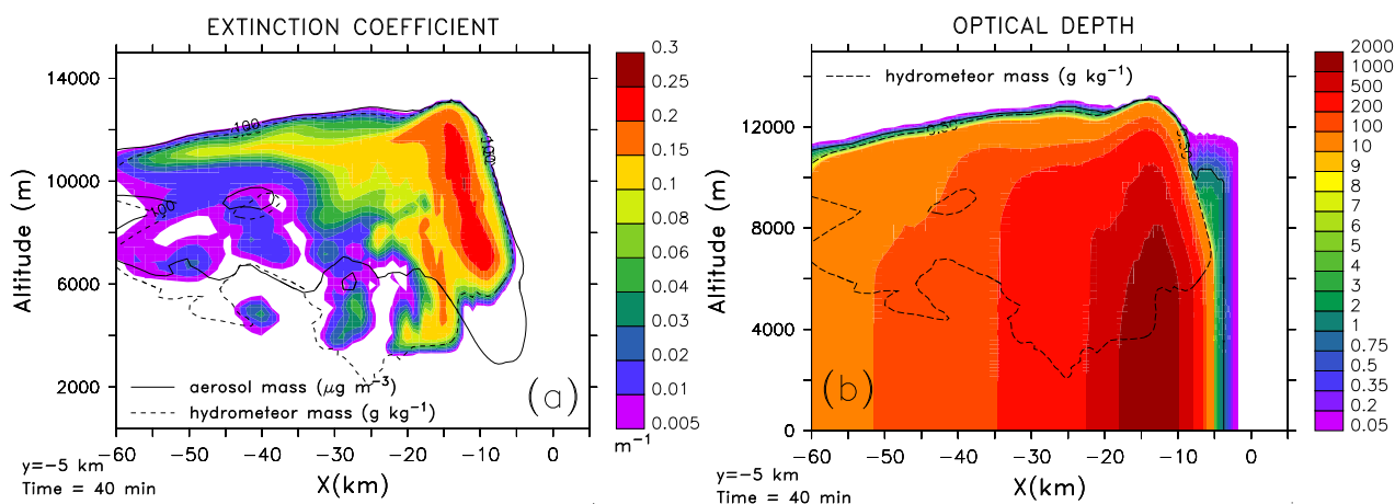
Fig. 6. Results from offline calculation of radiative properties. (a) Extinction due to absorption and scattering by hydrometeors and aerosols at 10.8 \mu\text{m} . Contours of aerosol mass concentration (solid line) and hydrometeor concentration (dashed line) indicate the extent of the smoke plume and pyroCb. (b) Aerosol and hydrometeor extinction optical depth \tau at 10.8 \mu\text{m} from the top of the atmosphere as a function of z . Note that the \tau=1 contour (solid line), which can be used as an indication of the effective level of emission of the thermal radiation, is situated very close to the cloud top.
