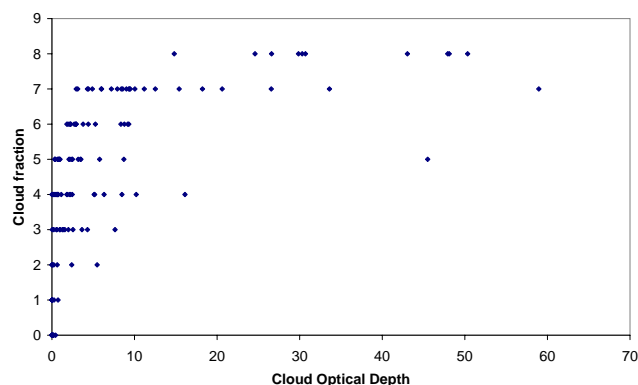
Fig. 2. Comparison of ground observations of cloudiness (cloud fraction in 1/8) (data from the Austrian Central Institute for Meteorology and Geodynamics ZAMG) with satellite determined cloud optical depth.
