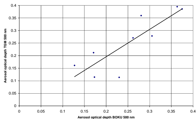
Fig. 4. Comparison of aerosol optical depth measurements at station BOKU (1) and at station TGM (3).
