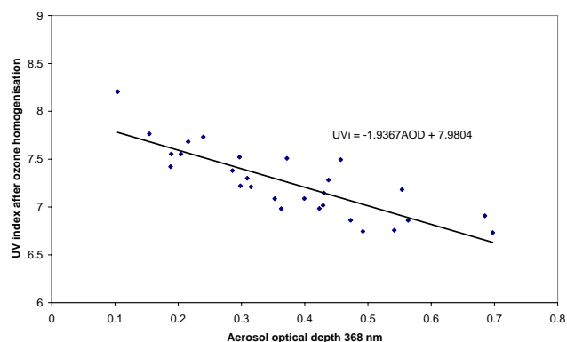
Fig. 5. Dependence of UV index on aerosol optical depth. A homogenisation was performed so that the UV index is referred to a column ozone value of 300 DU. Solar zenith angle is equal to 30 \pm 1^\circ .
