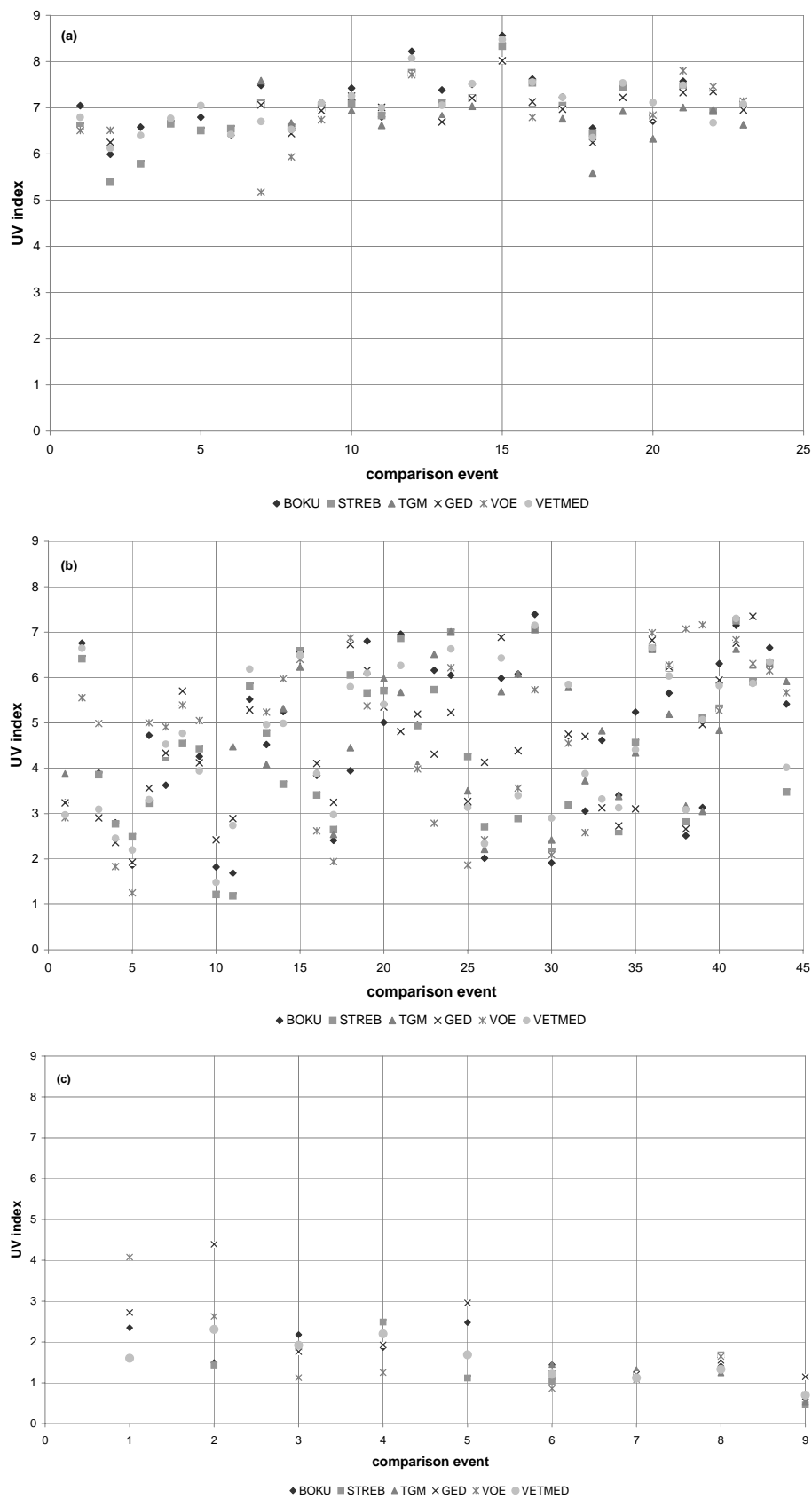
Fig. 3. Comparison of ground measurements performed at the 6 stations at noon during clear-sky conditions from May to July 2007.
