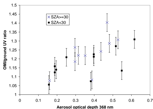
Fig. 8. Ratio of satellite retrieved to ground measured (BOKU station) erythemal UV for clear-sky conditions. The ratio is shown for solar zenith angles (SZA) larger and lower than 30^\circ . The errors bars correspond to the uncertainty of the OMI ratio, which results from the measurement uncertainty of the UV biometers.
