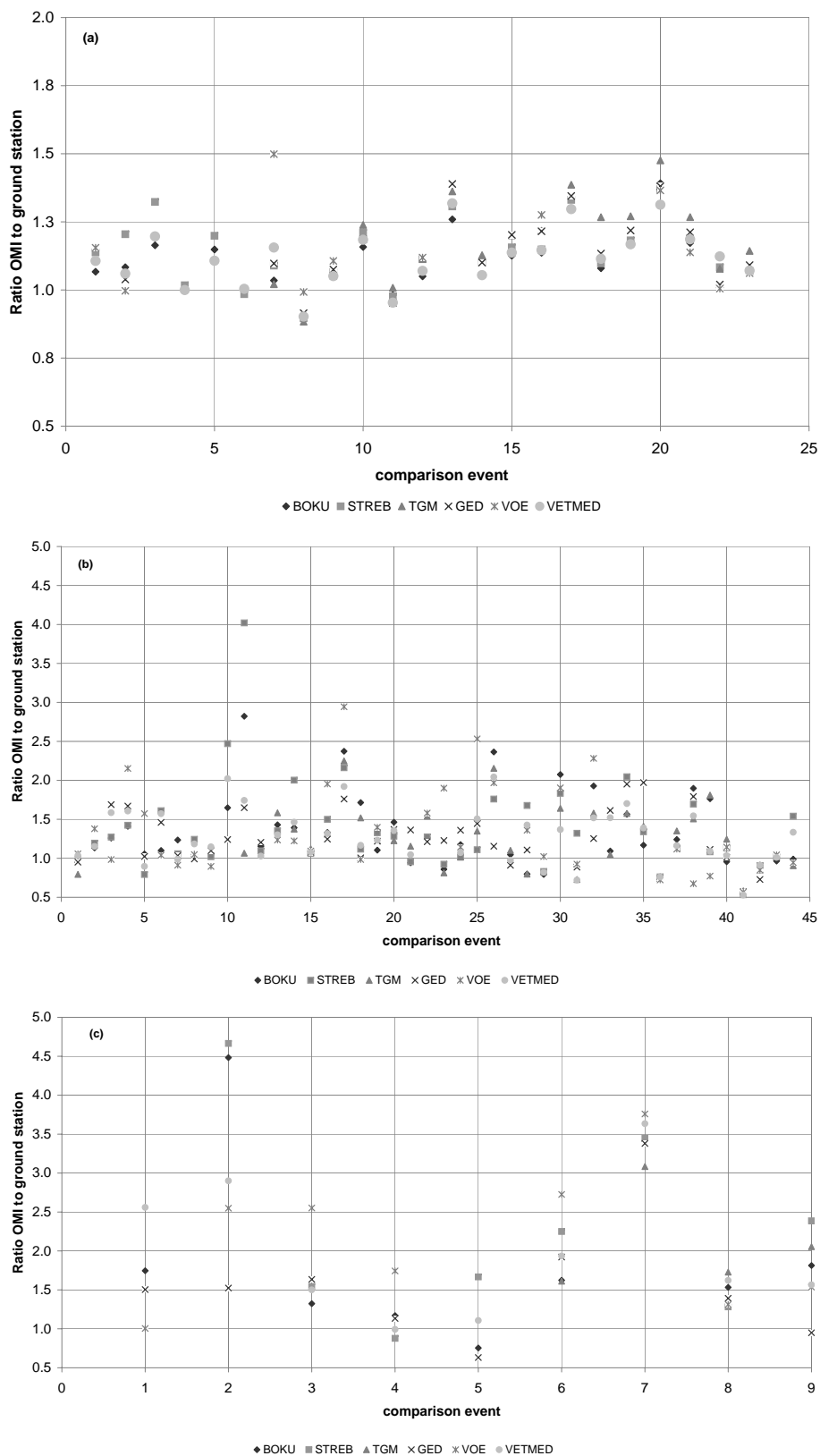
Fig. 7. Ratios of OMI observations to ground measurements during clear-sky (a), partly cloudy (b) and overcast conditions (c) from May to July 2007. Following results of Sect. 3.1, for the clear-sky comparisons instantaneous values and for cloudy conditions 1 h averages were used. STREB is for Strebersdorf, GED for Grossenzersdorf, VOE for Bad Voeslau and VETMED for University of Veterinary Medicine
