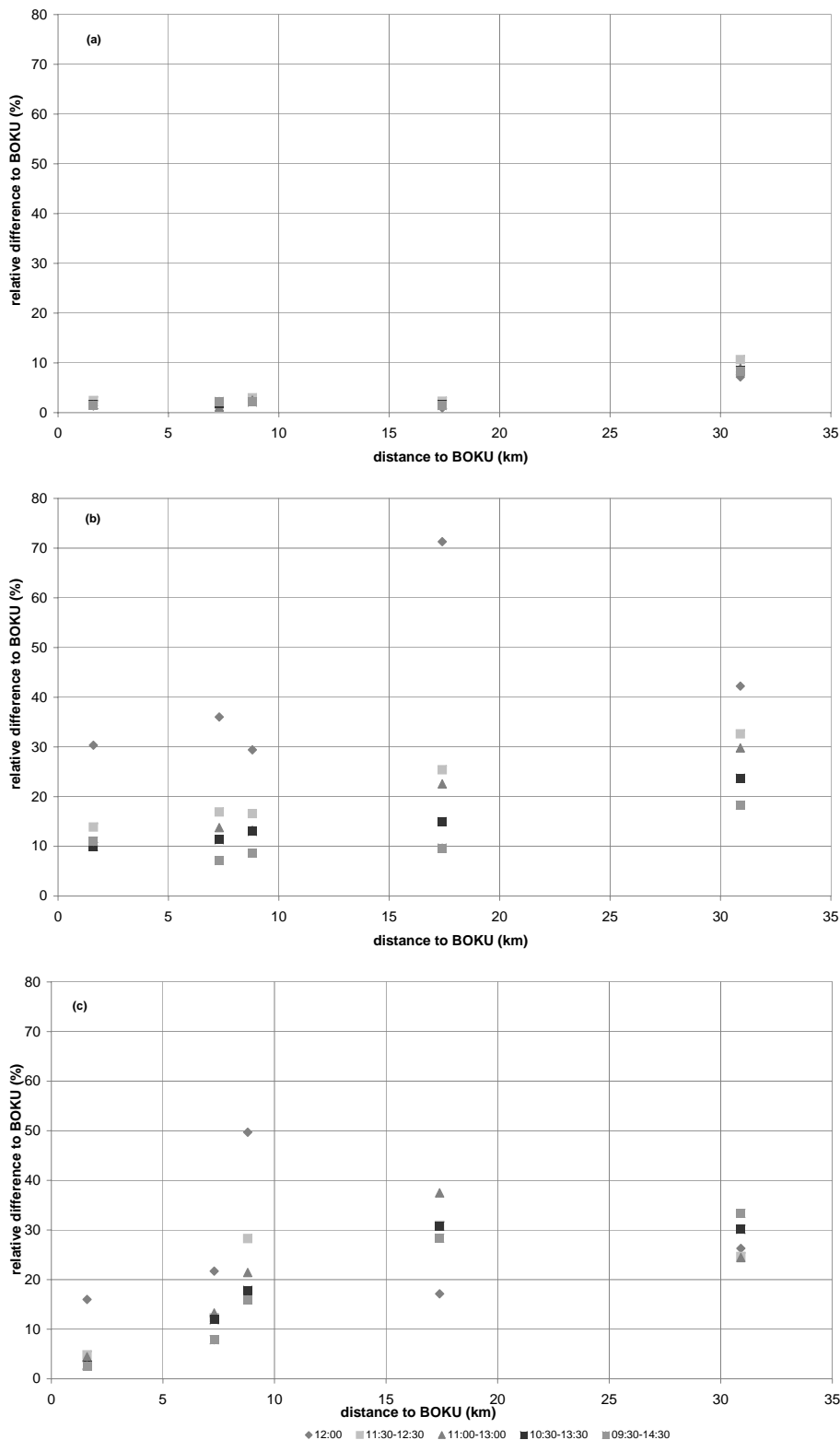
Fig. 6. Variability of UV index compared to BOKU UV index as a function of distance for different averaging intervals. Figure 6a shows variability for clear-sky, Fig. 6b for partly cloudy and Fig. 6c for overcast conditions. 12:00 is for instantaneous values, 11:30–12:30 is average from 11:30 Local solar time (LST) to 12:30 LST, 11:00–13:00 is average from 11:00 LST to 13:00 LST, 10:30–13:30 is average from 10:30 LST to 13:30 LST, 09:30–14:30 is average from 09:30 LST to 14:30 LST. The distances correspond to the stations as denoted in Table 3.
