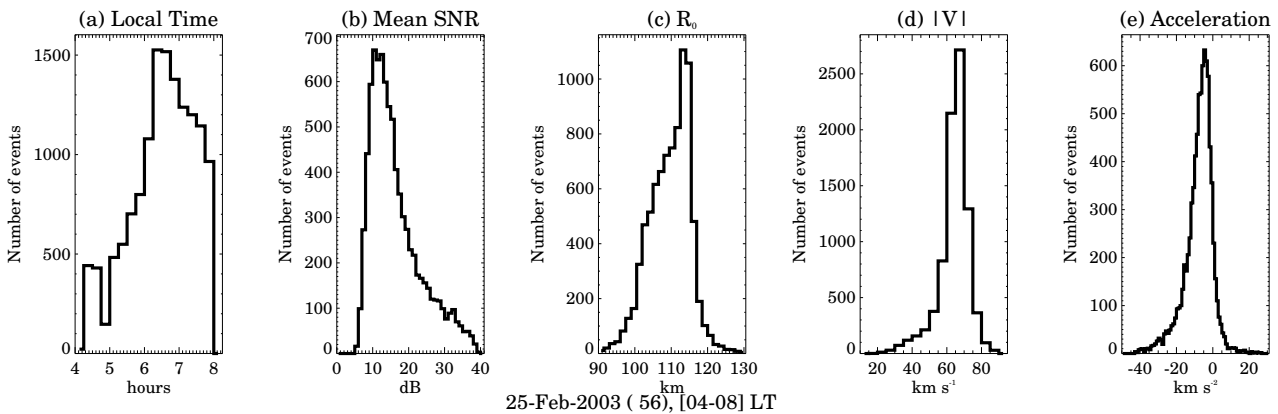
Fig. 6. Meteor statistics similar to Fig. 5 during a control night (when Leonid shower was not present) of 25 February 2003.
