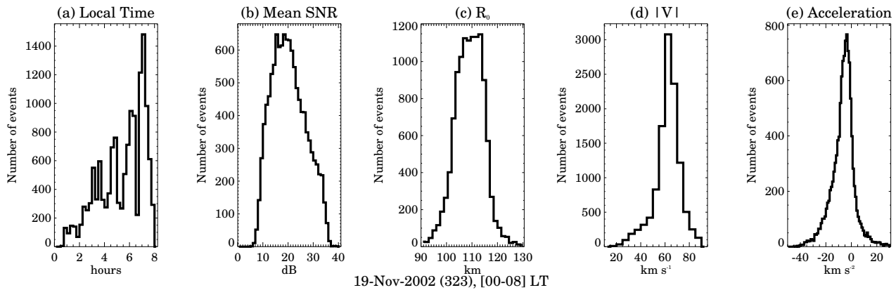
Fig. 5. Meteor statistics during 19 November 2002 when a Leonid shower occurred. (a) time, (b) mean SNR of meteor trajectory, (c) initial range, (d) absolute velocity, and (e) absolute acceleration.
