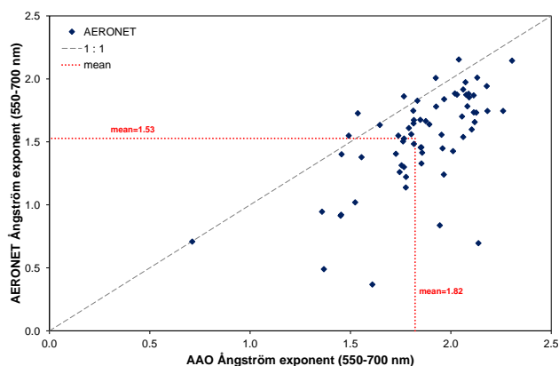
Fig. 3. Comparison of AAO aircraft calculated Ångström exponent with AERONET Ångström exponent (adjusted to 550–700 nm).
