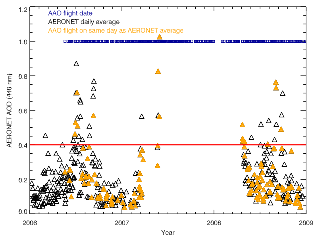
Fig. 1. Daily average of the AAO aircraft calculated aerosol optical depth and of the AERONET optical depth (at 440 nm) during the study period, and indicators of the days when AAO data are available.
