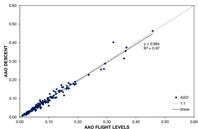
Fig. 16. Comparison of AAO aircraft calculated scattering optical depth adjusted to ambient RH for all the descent data with AAO scattering optical depth adjusted to ambient RH for the fixed sampling layers (at 550 nm).
