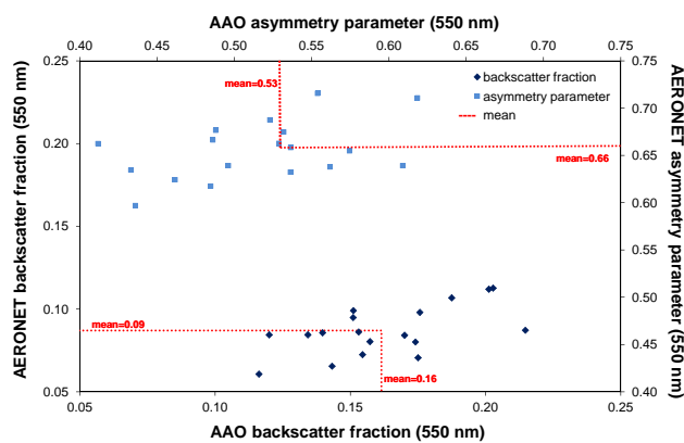
Fig. 4. Comparison of AAO aircraft calculated hemispheric backscatter fraction and asymmetry parameter with AERONET hemispheric backscatter fraction (calculated from the phase function and adjusted to 550 nm) and asymmetry parameter (adjusted to 550 nm).
