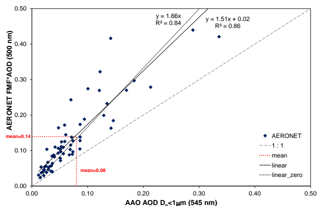
Fig. 11. Comparison of AAO aircraft calculated submicrometer AOD (at 545 nm) with AERONET Fine AOD (at 500 nm).
