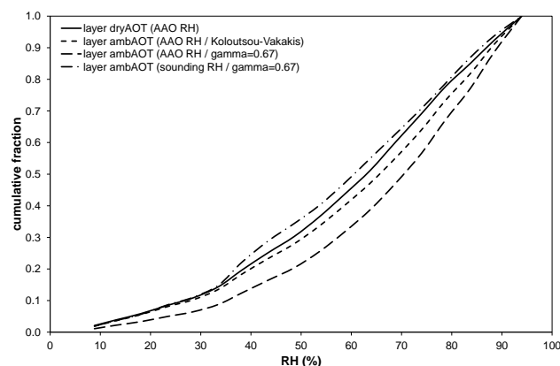
Fig. 10. Cumulative fraction of the AAO aerosol optical thickness for each flight level adjusted to low RH measured by the AAO RH sensor, the AAO aerosol optical thickness for each flight level adjusted to the ambient RH measured by the AAO RH sensor using both Koloutsou-Vakakis et al. (2001) ( \gamma = 0.33 ) and Quinn et al. (2005) ( \gamma = 0.67 ) parameterizations, and the AAO aerosol optical thickness for each flight level adjusted to the ambient RH measured by the atmospheric sounding using Quinn et al. (2005) parameterization ( \gamma = 0.67 ).
