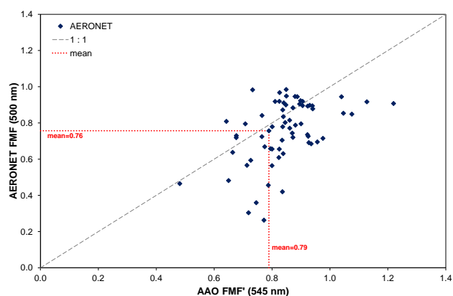
Fig. 5. Comparison of AAO aircraft calculated submicrometer Mode Fraction (at 545 nm) with AERONET Fine Mode Fraction (at 500 nm).
