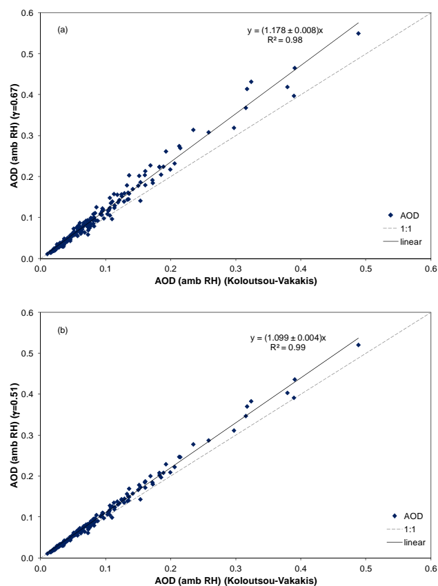
Fig. 9. Comparison of AAO aircraft calculated AOD adjusted to ambient RH using (a) Quinn et al. (2005) parameterization ( \gamma = 0.67 ) and (b) AAO f(\text{RH}) analysis ( \gamma = 0.51 ) with AAO AOD adjusted to ambient RH using Koloutsou-Vakakis et al. (2001) parameterization ( \gamma = 0.33 ) (at 550 nm).
