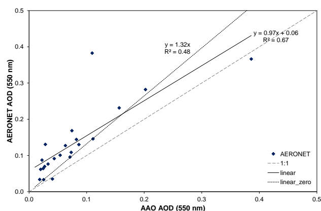
Fig. 6. Comparison of AAO aircraft calculated aerosol optical depth with AERONET optical depth (adjusted to 550 nm) for flights that have a RH < 60 % for all 11 levels.
