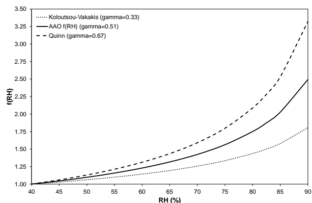
Fig. 8. Hygroscopic growth factor for light scattering, f(\text{RH}) , for Koloutsou-Vakakis et al. (2001) parameterization, Quinn et al. (2005) parameterization, and the limited AAO f(\text{RH}) analysis.
