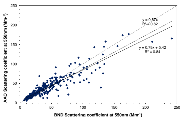
Fig. 12. Comparison of AAO averaged scattering coefficient from the lowest flight level over Bondville with the surface scattering coefficient averaged over the time of each profile.
