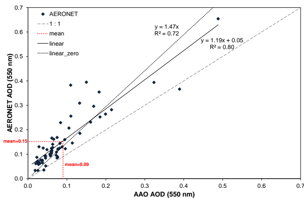
Fig. 2. Comparison of AAO aircraft calculated aerosol optical depth with AERONET optical depth (adjusted to 550 nm).
