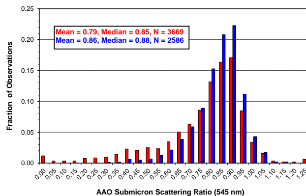
Fig. 13. Frequency distribution of AAO R_{SP} for all flight segments over Bondville (red) and for flight segments where the scattering coefficient was \geq 5 \text{ Mm}^{-1} (blue).
