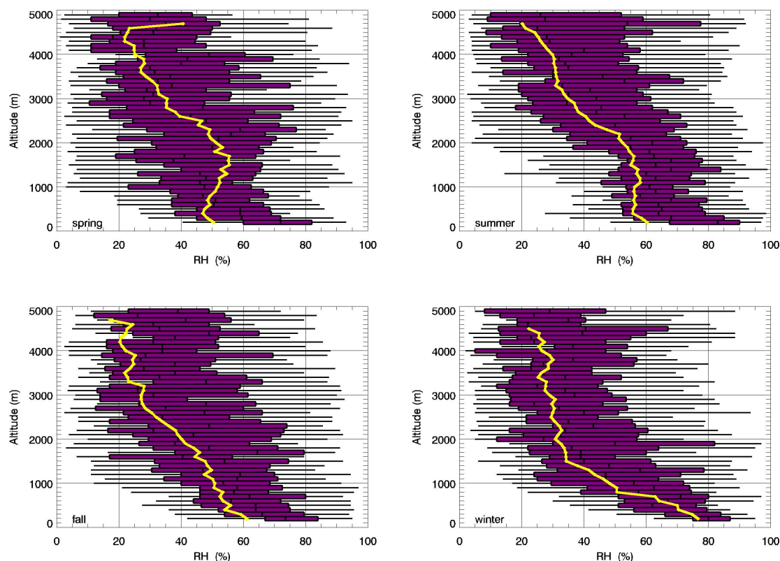
Fig. 7. Seasonal vertical profiles of the RH from the atmospheric soundings at Lincoln, Illinois, corresponding to AAO flights (box-whisker plots) and the median RH from the AAO flights (yellow line).
