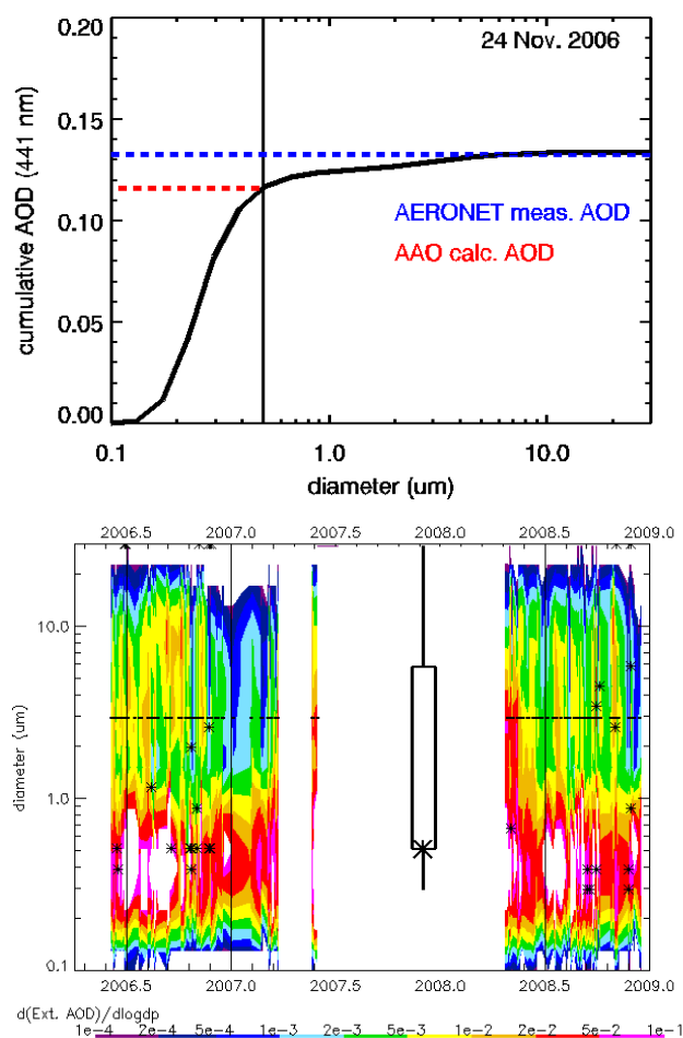
Fig. 14. (a) Cumulative AOD calculated from the AERONET measurements as a function of diameter for one AERONET size distribution retrieval. Vertical line represents the diameter where cumulative AERONET AOD matches AAO AOD; (b) Time series contour plot of AOD size distribution ( d(\text{AOD})/d\log D ) as a function of diameter. The color contours are based on AERONET volume size distribution retrievals and assumed refractive index as described in text. The asterisks (*) represent the diameter where the AAO AOD matches the cumulative AOD derived from AERONET size distributions (assuming \gamma = 0.67 for RH adjustment). The box-whisker diagram indicates statistics for the diameter for which the calculated cumulative AOD from the AERONET size distribution matches the AAO AOD. The ends of the whiskers are the 5th and 95th percentiles, the ends of the box are the 25th and 75th percentiles and the asterisk represents the median value (same as 25th percentile).
