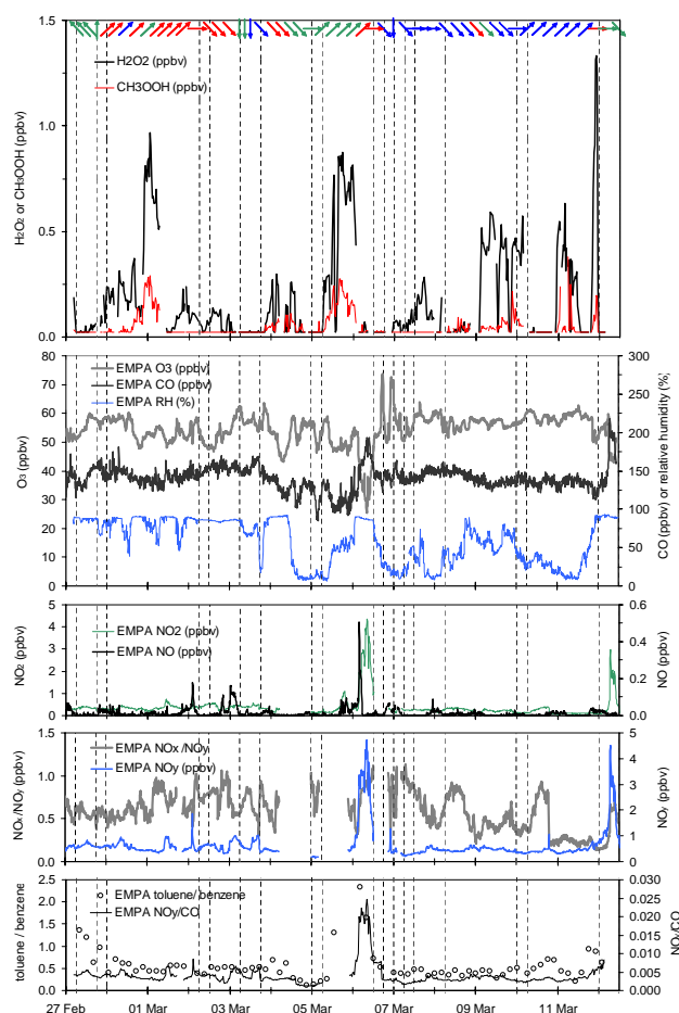
Fig. 4. Time series of \text{H}_2\text{O}_2 , \text{CH}_3\text{OOH} , \text{O}_3 , CO, relative humidity (RH), \text{NO}_2 , NO, \text{NO}_y , \text{NO}_x to \text{NO}_y , toluene to benzene and \text{NO}_y to CO ratios. Arrows in top panel and dashed vertical lines indicate changes in the prevailing wind direction deduced from the last day of 5-day back-trajectories (see Sect. 3.2 for further details). Descending air from >3.6 km (blue arrows), ascending air from <2 km (red arrows) and level (green arrows) indicates air that had remained at constant altitude for the last 5 days. Local NO and toluene contamination has been removed. Tick marks on time axis refer to noon (GMT).
