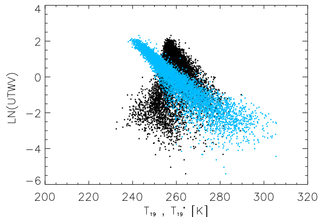
Fig. 7. As Fig. 6 but for AMSU-B channel 19.
