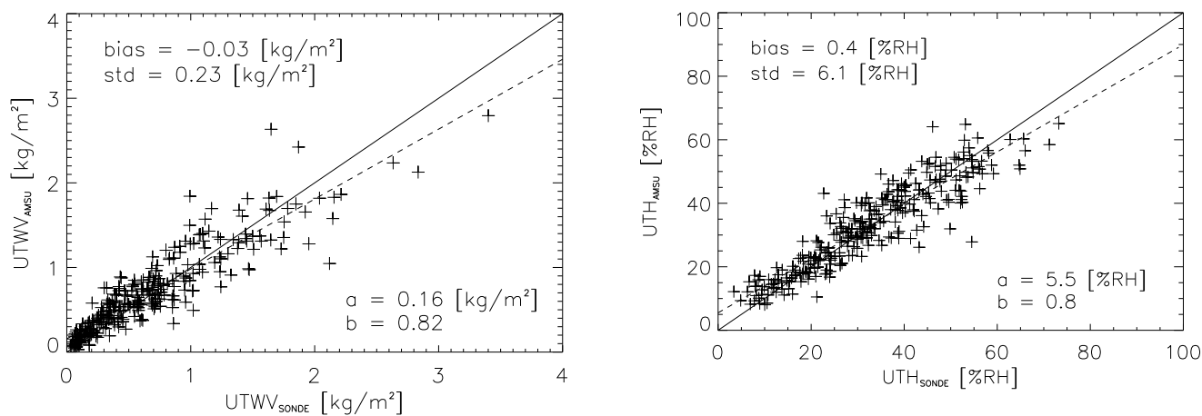
Fig. 15. As Fig. 14 but for the upper tropospheric humidity.
