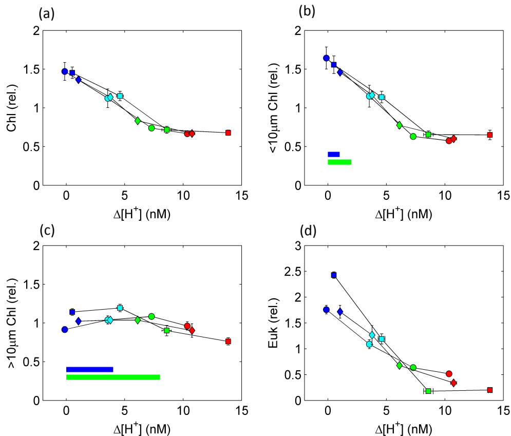
Figure 9. Relative changes in total (a), < 10 \mu\text{m} (b) and > 10 \mu\text{m} (c) size-fractionated Chl a and nano-/picoeukaryotes counts (d) as a function of the change in [\text{H}^+] after 48 h incubation in three (E3–E5) out of the five main bioassay experiments. Data for each variable are normalised to the mean value for this time point and plotted against the difference in [\text{H}^+]^{\text{bulk}} between the ambient incubation and the treatment. Values plotted are mean \pm 1 SE for both axes. Solid bars in (b) and (c) indicate approximate ranges of cell surface ( [\text{H}^+]^{\text{prox}} ) which might be experienced by small and large cells over short timescales, i.e. hours–days (see Kuhn and Raven 2008; Flynn et al., 2012), under ambient modern conditions (blue) and at \sim 750 \mu\text{atm} (green) (Flynn et al., 2012). Colours indicate treatment conditions as in Fig. 7.
