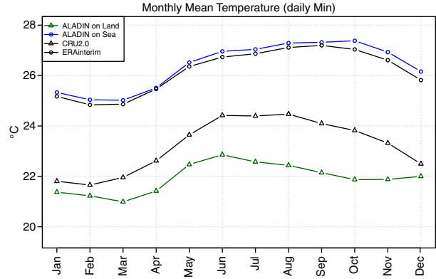
Fig. 4. Monthly mean T_{\min} (minimum daily temperature) over the area 12\text{--}20^\circ\text{N} and 56\text{--}64^\circ\text{W} , obtained from ERA-interim dataset in black with circles (median on 156 sea points), CRU2.0 dataset in black with triangles (median on 28 land points), ALADIN simulation on Land in green with triangles (median on 47 land points), ALADIN simulation on Sea in blue with circle (median on 7128 sea points) for the end of the 20th century. Units are in ^\circ\text{C} .
