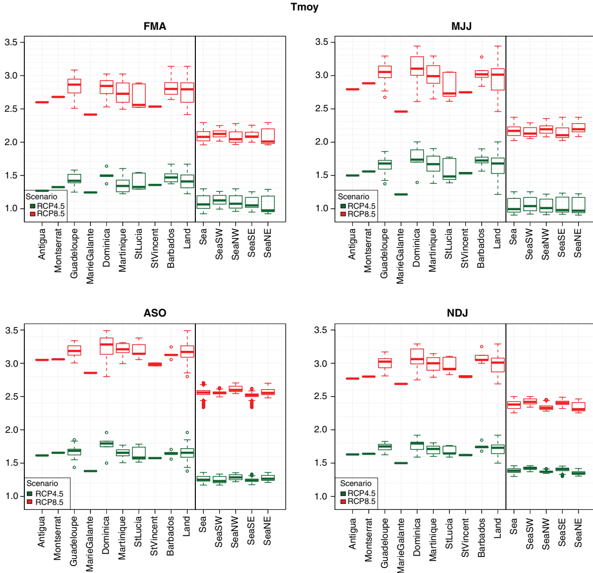
Fig. 5. Projections of the seasonal mean temperature for the period 2071–2100 relative to the period 1971–2000 baseline under two scenarios (RCP4.5 in green and RCP8.5 in red) over all islands and Sea (divided in four zones: NW, NE, SE, SW). Units are in °C.
