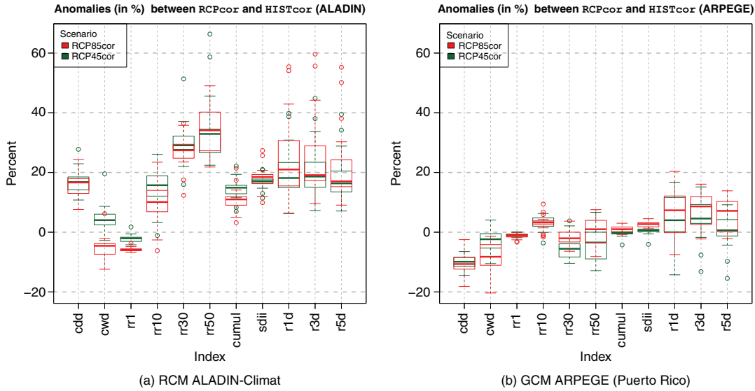
Fig. 8. Anomalies of indexes between HISTCOR and RPCOR in percentage.
