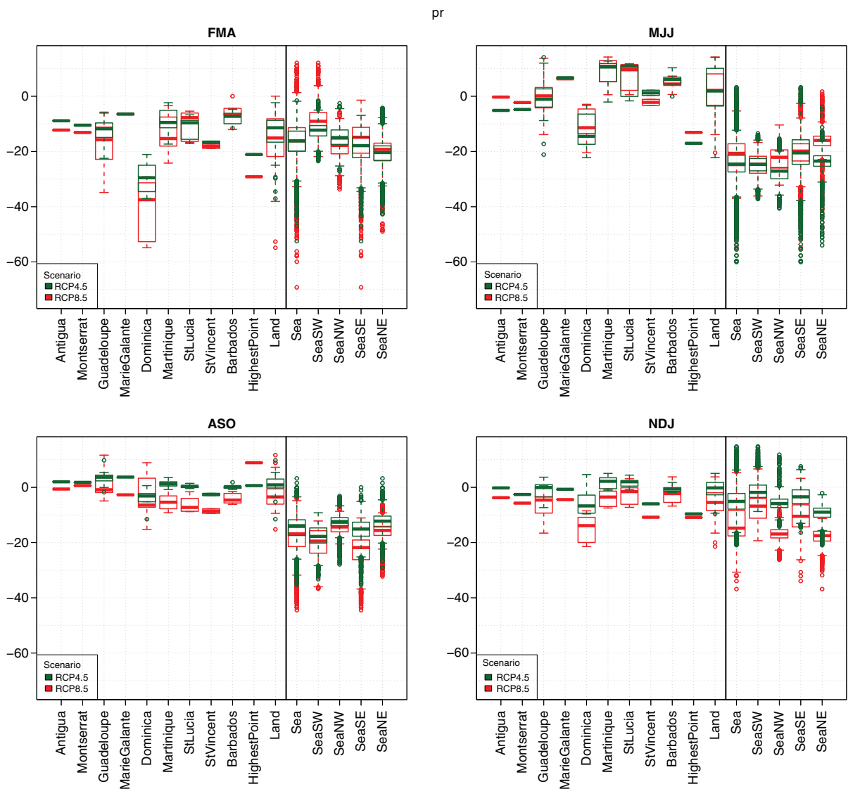
Fig. 6. Projections of the seasonal mean precipitation for the period 2071–2100 relative to the period 1971–2000 baseline underline two scenarios (RCP4.5 in green and RCP8.5 in red) over all islands and Sea (divided in four zones: NW, NE, SE, SW). Units are in %.
