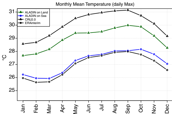
Fig. 3. Monthly mean T_{\max} (maximum daily temperature) over the area 12\text{--}20^\circ\text{N} and 56\text{--}64^\circ\text{W} , obtained from ERA-interim dataset in black with circles (median on 156 sea points), CRU2.0 dataset in black with triangles (median on 28 land points), ALADIN simulation on Land in green with triangles (median on 47 land points), ALADIN simulation on Sea in blue with circle (median on 7128 sea points) for the end of the 20th century. Units are in ^\circ\text{C} .
