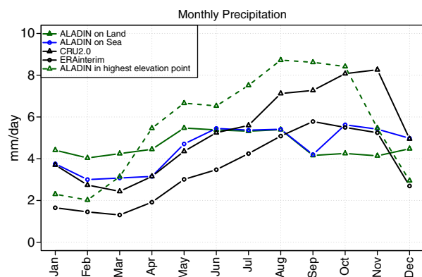
Fig. 2. Monthly mean precipitation over the area 12–20°N and 56–64°W, obtained from ERA-interim dataset in black with circles (median on 156 sea points), CRU2.0 dataset in black with triangles (median on 28 land points), ALADIN simulation on Land in green with triangles (median on 47 land points), ALADIN simulation on Sea in blue with circle (median on 7128 sea points) for the end of the 20th century. Units are in mm/day.
