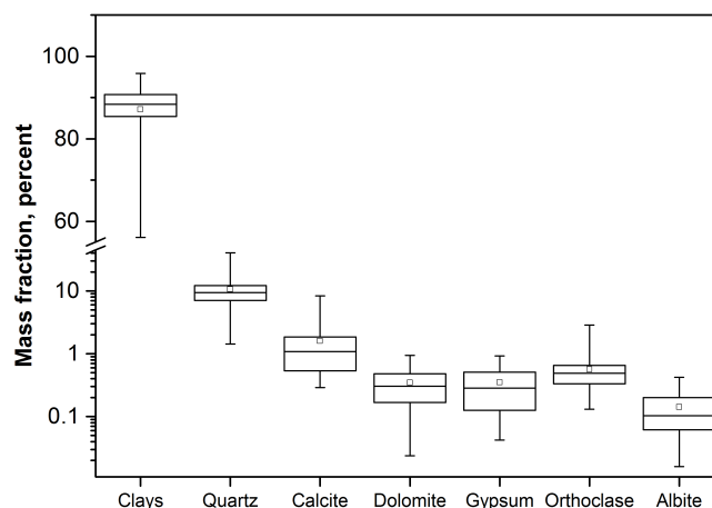
Figure 4. Range of variability of the mineral content (in percent) as obtained by XRD analysis. Boxes indicate the 25, 50 and 75 % percentiles. Whiskers indicate the minimum and the maximum values, whereas the open squares indicate the mean value of the distribution.
