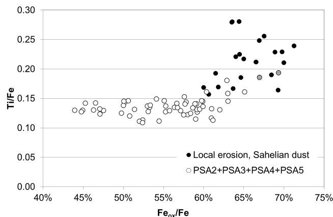
Figure 8. Scatter plot of the Ti/Fe ratio with respect to the \text{Fe}_{\text{ox}} -to-Fe ratio.
