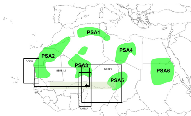
Figure 2. Geographical identification of the origin of the analysed samples superimposed on the localisation of the major potential source areas (PSA, in green) of mineral dust in western and northern Africa proposed by Formenti et al. (2011a) and Scheuven et al. (2013) on the basis of the analysis of satellite products and the chemical/mineralogical composition of the aerosol and the parent soil. The approximate localisation of the Sahelian dust sources is also indicated by the shaded light green area. The location of the Banizoumbou ground-based site is indicated by the black cross. The operating areas of the AMMA, DABEX, DODO and GERBILS field projects are shown by black boxes. Figure reproduced from Scheuven et al. (2013) with permission from Elsevier.
