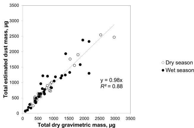
Figure 1. Comparison between the total estimated dust mass (TEDM) estimated from the chemical composition and the total dry gravimetric mass (TDGM) for the AMMA SOP0 (dry season, open circles) and AMMA SOP1-2 data (wet season, black circles). The dashed line represents the slope of the calculated linear regression.
