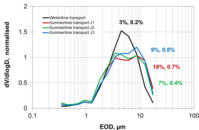
Figure 9. Normalised volume size distribution dV/d\log (equivalent optical diameter, EOD) at Banizoumbou during 3 consecutive days in summer (labelled J1 (red line), J2 (green line) and J3 (blue line)) and one day in winter (black line) for samples representing dust transported from the Bodélé source region. Data are reported as a function of the EOD as obtained by optical counter measurements without any corrections for the sample refractive index.
