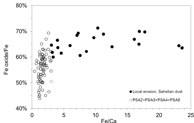
Figure 6. Dependence of the \text{Fe}_{\text{ox}} content ( \text{Fe}_{\text{ox}} -to-Fe ratio) on the Fe/Ca ratio for samples of different source regions identified in this study.
