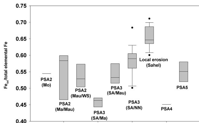
Figure 5. Variability of the iron oxide content (ratio of \text{Fe}_{\text{ox}} to total elemental Fe) according to the source region. Boxes indicate the 25, 50 and 75 % percentiles. Whiskers indicate the minimum and the maximum values, and points indicate the 5 and 95 % percentiles. Data labels are as follows: Mo stands for Morocco; Ma stands for Mali; Mau stands for Mauritania; SA stands for southern Algeria; and NN stands for northern Niger.
