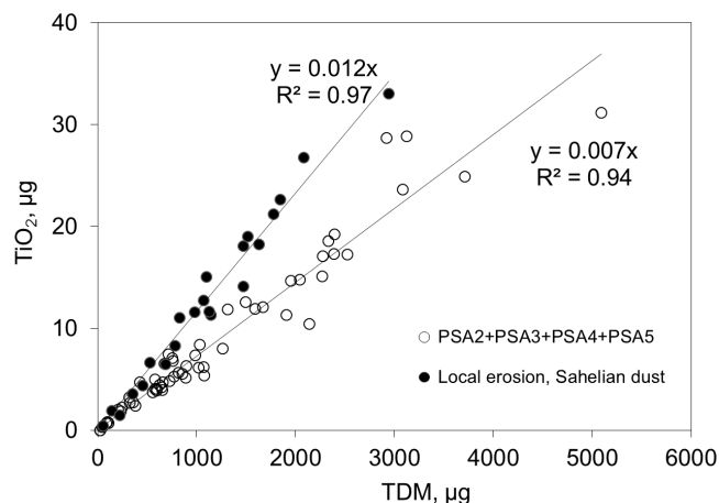
Figure 7. Scatter plot of the estimated mass of \text{TiO}_2 with respect to the total dust mass (TDM). Open circles are used to display values for samples corresponding to transport of Saharan dust, whereas filled circles are for samples corresponding to local emission in the Sahel.
