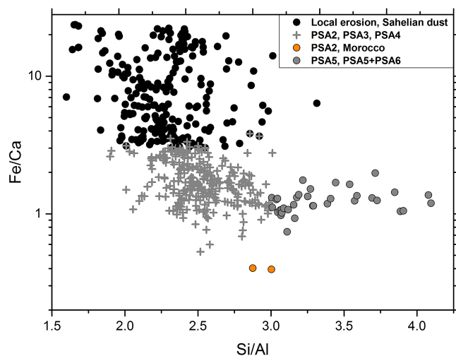
Figure 3. Scatter plot of the elemental ratio Fe/Ca versus Si/Al with additional information on source identification based on back trajectory, satellite and dispersion modelling.
