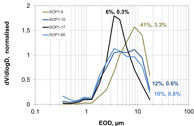
Figure 10. Normalised volume size distribution dV/d\log(EOD) for samples representing emitted dust in the Sahel during episodes of local erosions. The explanation of the sample ID is given in the text.
