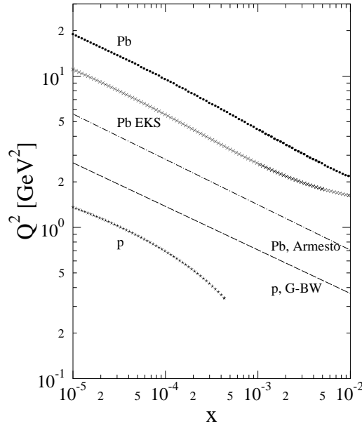
Fig. 2: The gluon saturation limits in the DGLAP+GLRMQ approach for proton (asterisks) and Pb ( A = 208 ), with (crosses) and without (dots) nuclear modifications [8]. The saturation line for the proton from the geometric saturation model [11] (dashed line), and for Pb from [12] (dotted-dashed) are also plotted.
