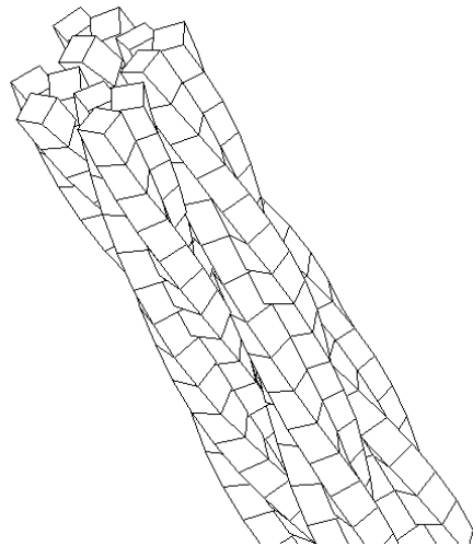
Figure 4. Detail of the geometry generated for a 3x4 cable with the cross section shown in Fig. 2. Note the inversion in the twisting direction between first and second stage.
