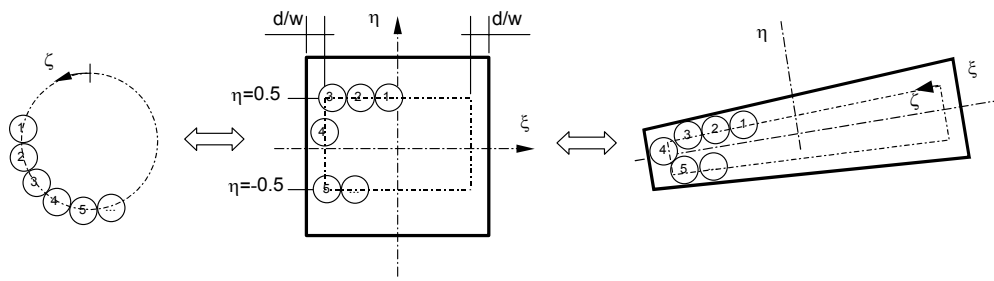
Figure 3. Principle for randomized meshing of a cable. The first strand is placed randomly on the \zeta circle, the following strands are equispaced. This distribution is then mapped first in the parent plane and afterwards in the physical plane.
