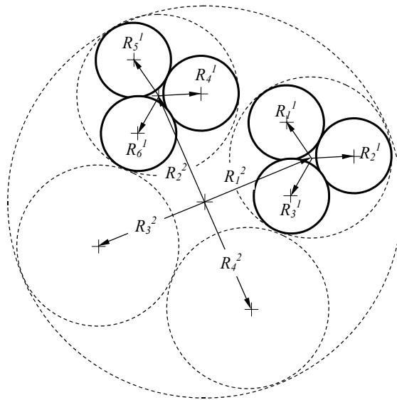
Figure 2. Definition of the polar coordinates of the sub-elements of a 3x4x4 cable in the reference plane. Only two triplets (stage 1) are shown for clarity.
