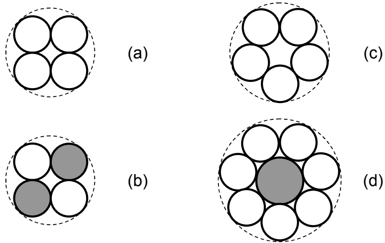
Figure 1. Cabling patterns considered for a sub-cable stage: (a) a n-plet of superconducting strands, (b) an hybrid of superconducting strands and pure stabilizer strands, (c) a hollow cable and (d) cable around a core with different diameter and material (e.g., pure stabilizer).
