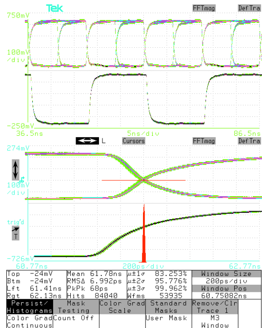
Figure 6: PCR transmitter encoder jitter
