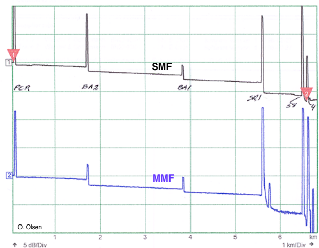
Figure 3: OTDR PCR – B4
