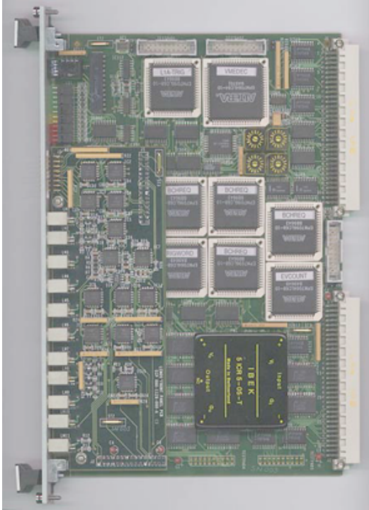
Figure 13: TTCvi VMEbus interface
