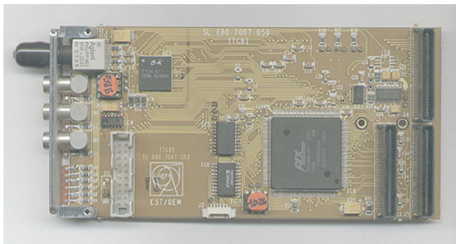
Figure 24: TTCbi PMC module
