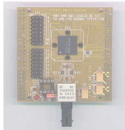
Figure 21: TTCrm mezzanine board
